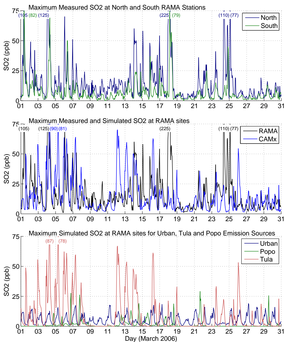
Fig. 2. Measured and simulated SO 2 in the MCMA. Maximum 1-hour concentrations for the North and South station groups defined in Fig. 1 (Top). Comparison of maximum domain-wide RAMA measurements and CAMx simulations (Middle). Domain-wide maximum of CAMx simulations for all RAMA stations measuring SO 2 , for separate source groups (Bottom). Maximum of values off the chart shown in brackets.
