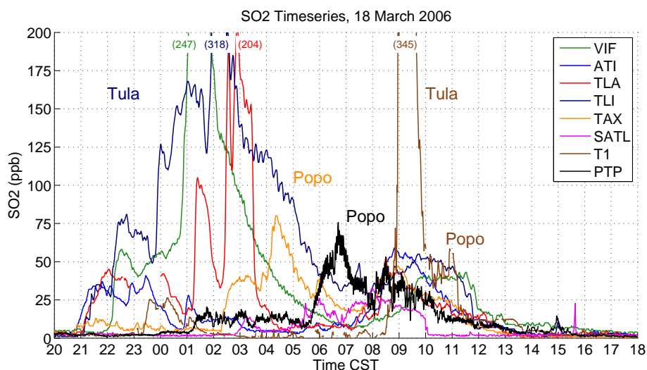
Fig. 17. Time series of measured SO 2 concentrations for 18 March. Maximum of values off the chart shown in brackets. Tula and Popo plumes labelled with the colour of the corresponding site.
