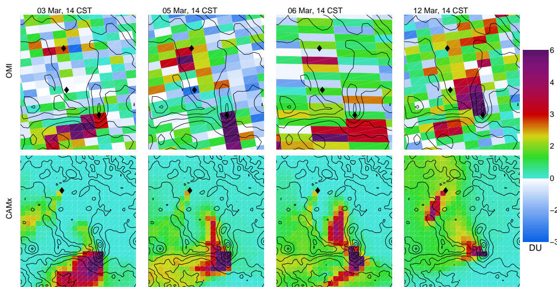
Fig. 4. SO 2 total columns from OMI swath data and CAMx regional simulations with 9 by 9 km grid cells with all sources (urban, Tula and Popocatepetl). Black diamonds shows the location of Tula and Popo. Terrain contours every 500 m.
