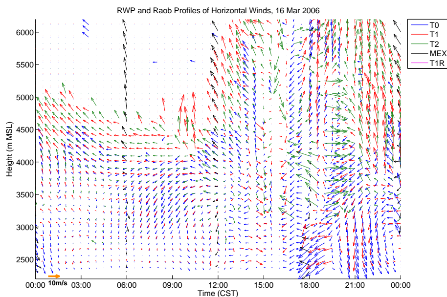
Fig. 14. Radar wind profiler and Radiosonde wind vectors at GSMN, T0, T1 and T2 on 16 March 2006. This shows the evolution of horizontal winds with height, an arrow pointing up means winds moving north. MEX are the radiosondes launched at GSMN, T1R are the radiosondes launched at T1.
