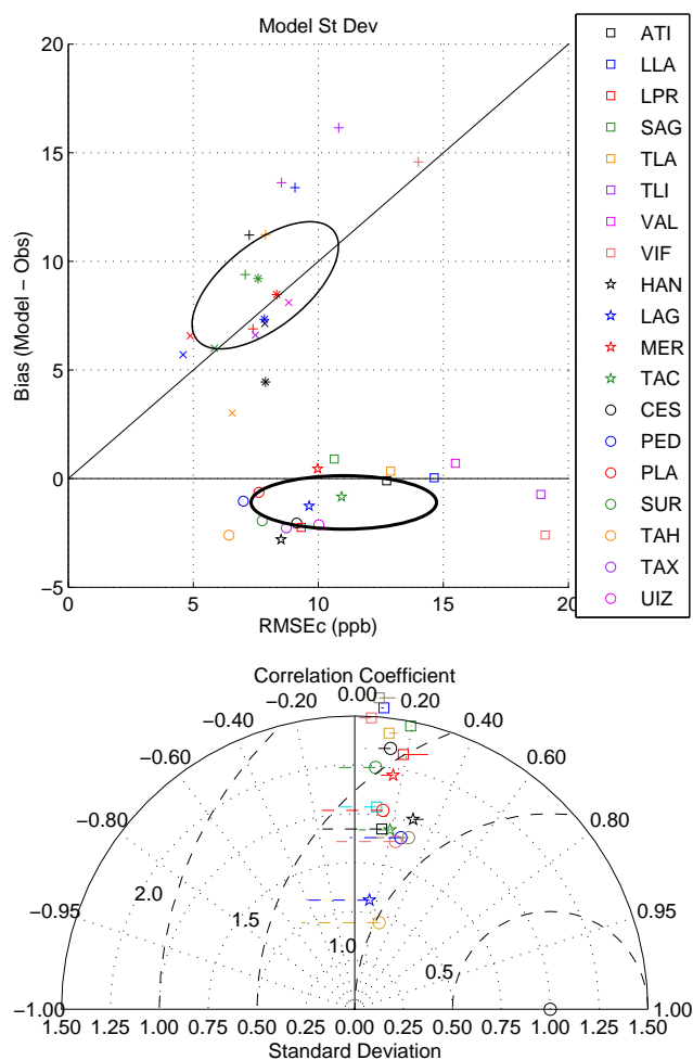
Fig. 3. Statistics diagrams of simulated versus measured hourly SO 2 by station in the MCMA. Top: RMSEc-bias diagram, open symbols show the model bias versus the centred root mean square error (RMSEc). Closed symbols show the model standard deviation versus that of the observations (squares match '+', circles match 'x'). Ellipses are centred on the mean with semi-axes given by the standard deviations of the metrics. Bottom: Taylor diagram showing the correlation coefficient and the standard deviation, solid horizontal line indicates positive bias, dashed line for negative bias.
