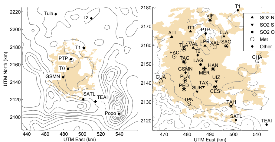
Fig. 1. Map of the basin and the MCMA showing sites used in this study. RAMA SO 2 and meteorology sites shown on the right, classified by groups used for plotting (N=North, S=South, O=Central). Urban area of the MCMA shown in beige, terrain contours every 250 m.
