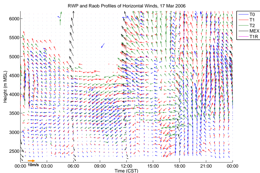
Fig. 16. Radar wind profiler and Radiosonde wind vectors at GSMN, T0, T1 and T2 on 17 March 2006. This shows the evolution of horizontal winds with height, an arrow pointing up means winds moving north. MEX are the radiosondes launched at GSMN, T1R are the radiosondes launched at T1.
