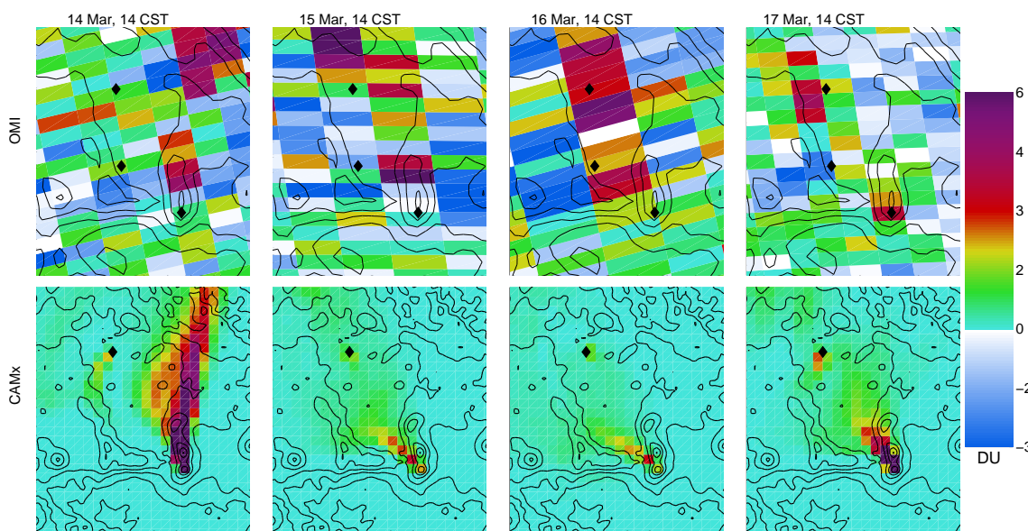
Fig. 5. SO 2 total columns from OMI swath data and CAMx regional simulations with 9 by 9 km grid cells with all sources (urban, Tula and Popocatepetl). Black diamonds shows the location of Tula and Popo. Terrain contours every 500 m.
