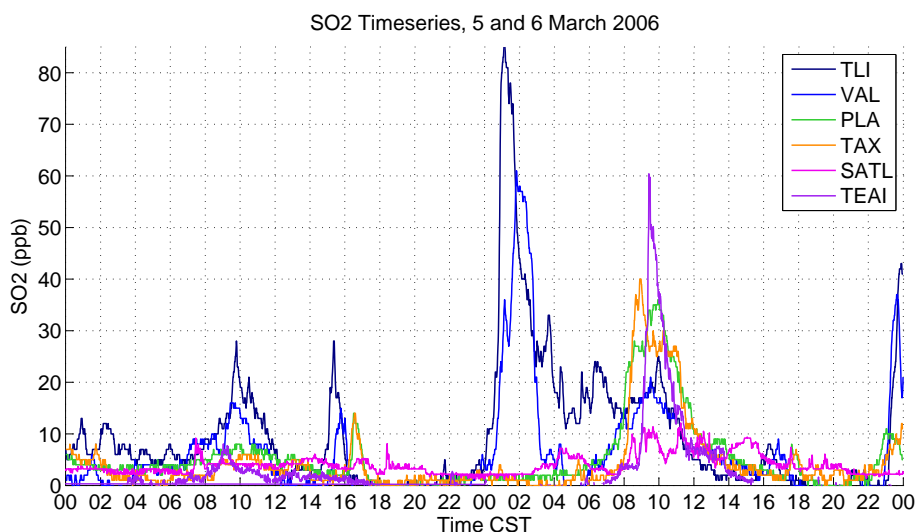
Fig. 9. Time series of measured SO 2 concentrations for 5 and 6 March.
