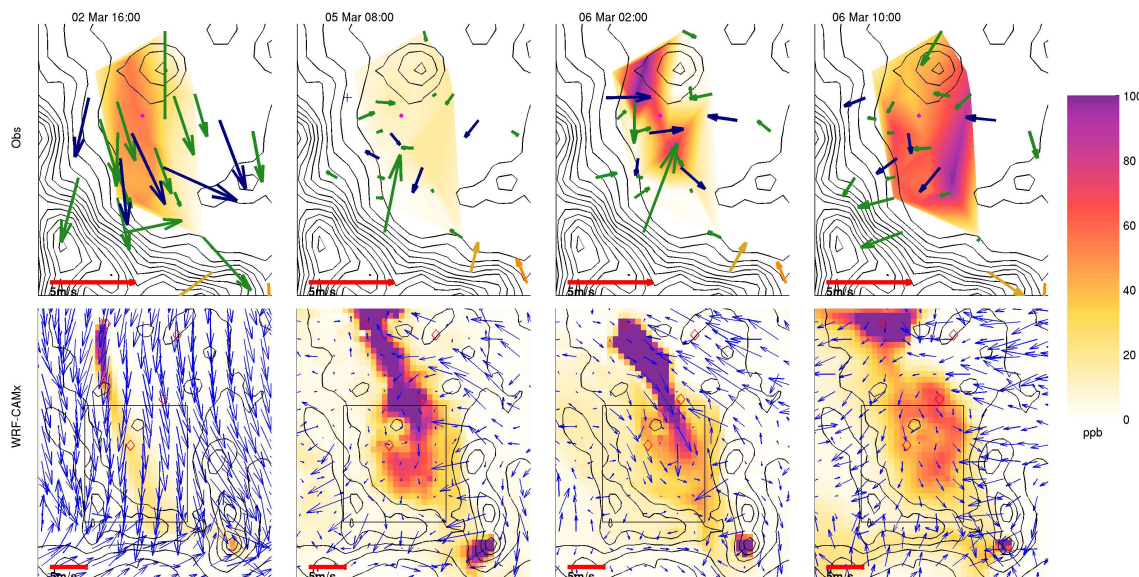
Fig. 8. Measured winds and hourly surface concentration of SO 2 in the MCMA and simulated winds (WRF) and SO 2 (CAMx, all sources) in the basin. Observed winds are coloured according to network: green - RAMA, blue - SMN, magenta - T1, tan - St. Ana, orange - Tenango del Aire. Terrain contours every 100 m (top) and 500 m (bottom), measurement domain shown as a box in model domain, red diamonds show T0, T1, T2 and Tula.
