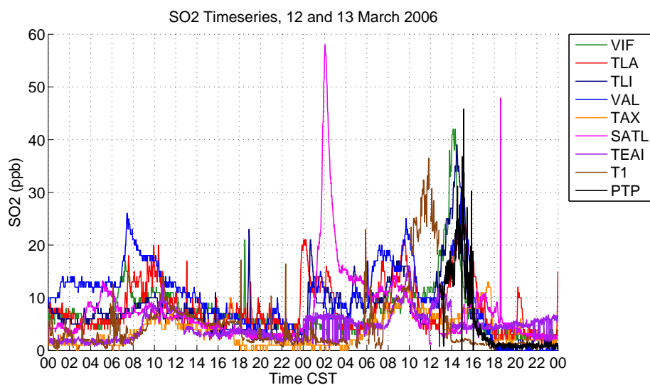
Fig. 10. Time series of measured SO 2 concentrations for 12 and 13 March.
