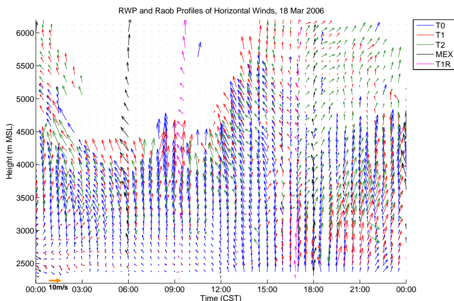
Fig. 18. Radar wind profiler and Radiosonde wind vectors at GSMN, T0, T1 and T2 on 18 March 2006. This shows the evolution of horizontal winds with height, an arrow pointing up means winds moving north. MEX are the radiosondes launched at GSMN, T1R are the radiosondes launched at T1.
