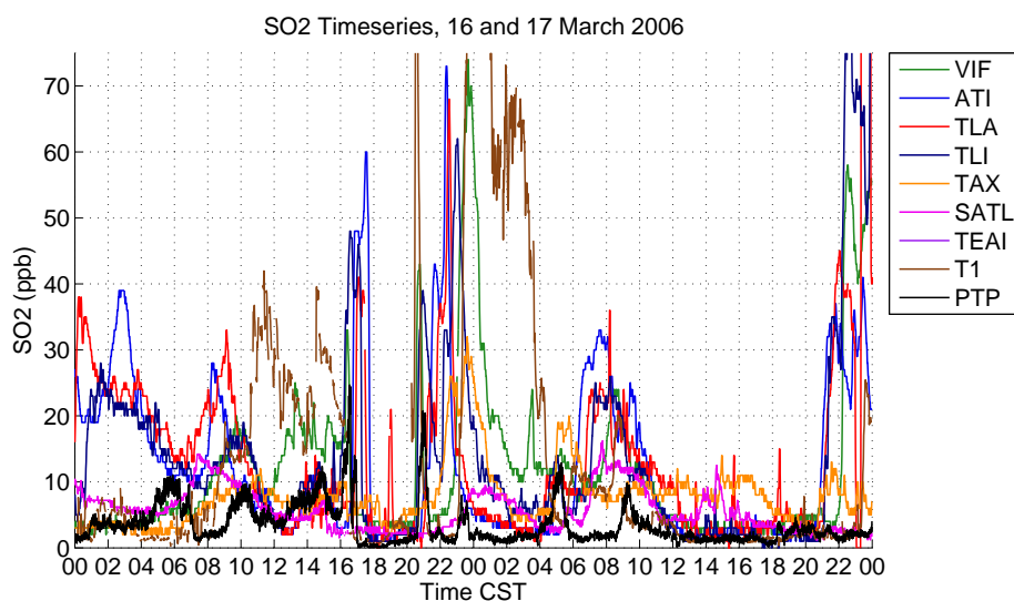
Fig. 13. Time series of measured SO 2 concentrations for 16 and 17 March.
