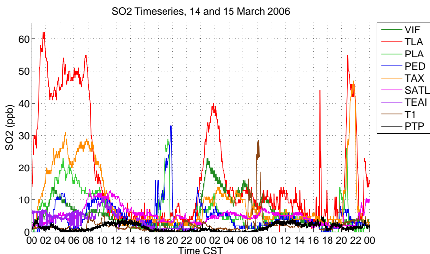
Fig. 12. Time series of measured SO 2 concentrations for 14 and 15 March.
