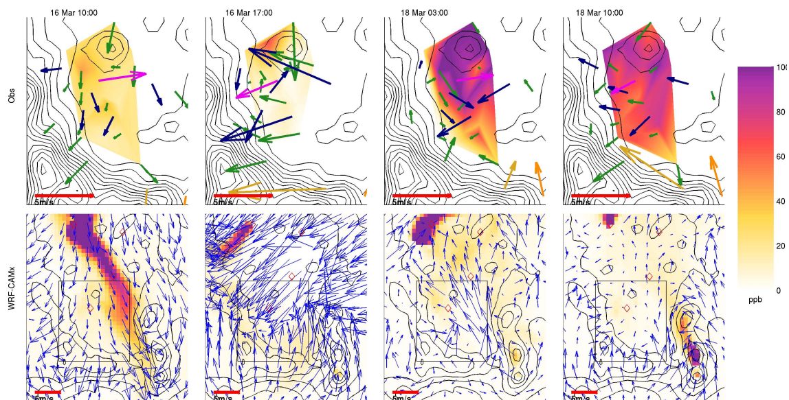
Fig. 15. Measured winds and hourly surface concentration of SO 2 in the MCMA and simulated winds (WRF) and SO 2 (CAMx, all sources) in the basin. Observed winds are coloured according to network: green - RAMA, blue - SMN, magenta - T1, tan - St. Ana, orange - Tenango del Aire. Terrain contours every 100 m (top) and 500 m (bottom), measurement domain shown as a box in model domain, red diamonds show T0, T1, T2 and Tula.
