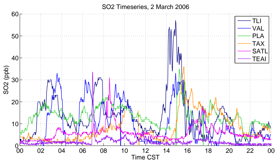
Fig. 7. Time series of measured SO 2 concentrations for 2 March.
