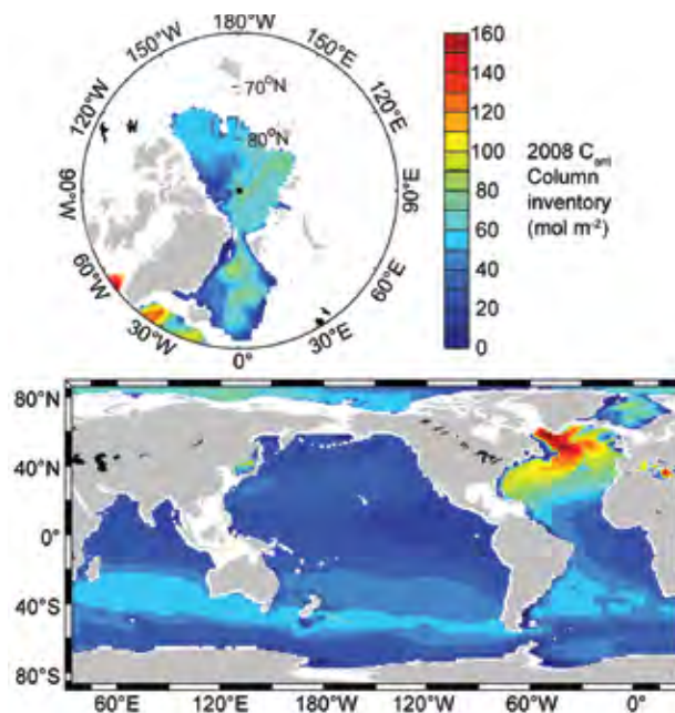
FIG. 3.33. Compilation of 2008 column inventories ( \text{mol m}^{-2} ) of anthropogenic \text{CO}_2 ( C_{\text{ant}} ): the global Ocean excluding the marginal seas (Khatiwala et al. 2009), 140 \pm 25 Pg C; Arctic Ocean (Tanhua et al. 2009) 2.6 Pg C–3.4 Pg C; the Nordic seas (Olsen et al. 2010) 1.0 Pg C–1.5 Pg C; the Mediterranean Sea (Schneider et al. 2010) 1.5 Pg C–2.4 Pg C; the East Sea (Sea of Japan; Park et al. 2006) 0.40 \pm 0.06 Pg C. All the marginal sea estimates were computed for 1994 and then scaled to 2008 assuming transient steady state storage of anthropogenic carbon ( C_{\text{ant}} ).
