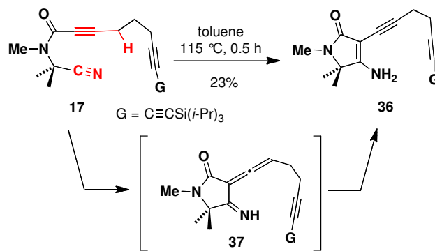
Scheme 4. Evidence for Propargylic Cyano Ene Reaction: Isolation of Enamine 36
