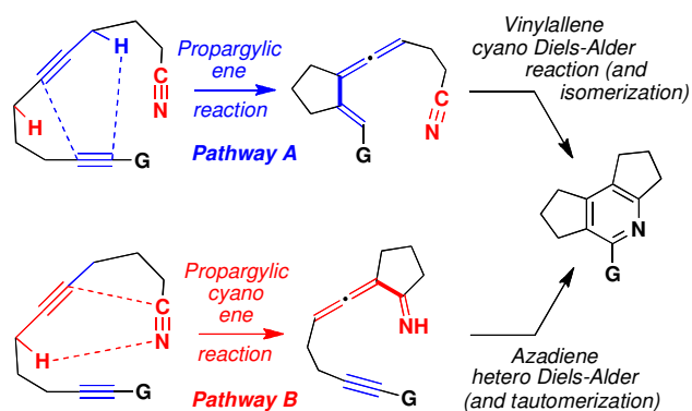
Scheme 1. Synthesis of Pyridines via Pericyclic Cascade Strategies
