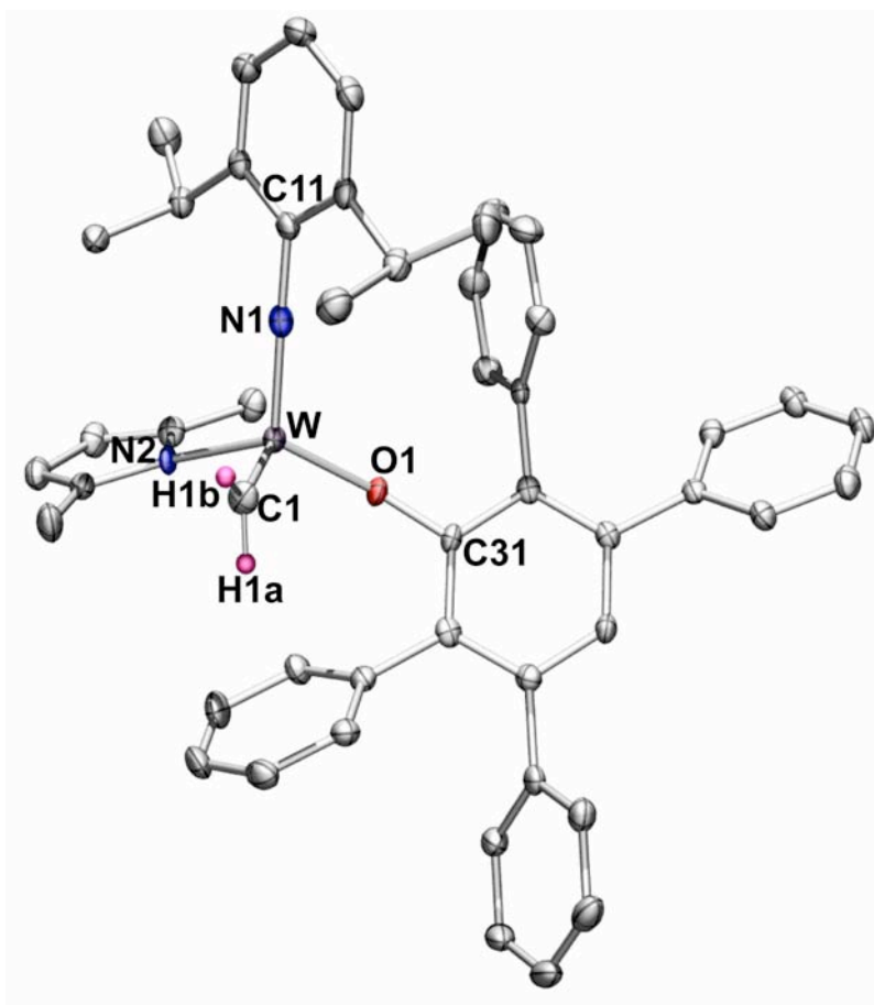
Figure 1. A thermal ellipsoid drawing of W(NAr)(CH_2)(OTTP)(Me_2Pyr) ( 2 w ) (50% probability). Hydrogen atoms except for those on the methylene are removed for clarity. Selected bonds (Å) and angles (°): W-N1 = 1.758(4) , W-N2 = 2.020(4) , W-O1 = 1.913(3) , W-C1 = 1.908(4) , W-N1-C11 = 176.8(3) , W-O1-C31 = 148.4(3) , W-C1-H1a = 107(4) , W-C1-H1b = 136(3) , H1a-C1-H1b = 117(5) . The angle between planes through H1a-C1-H1b and N1-W-C1 is 7.7^\circ .
