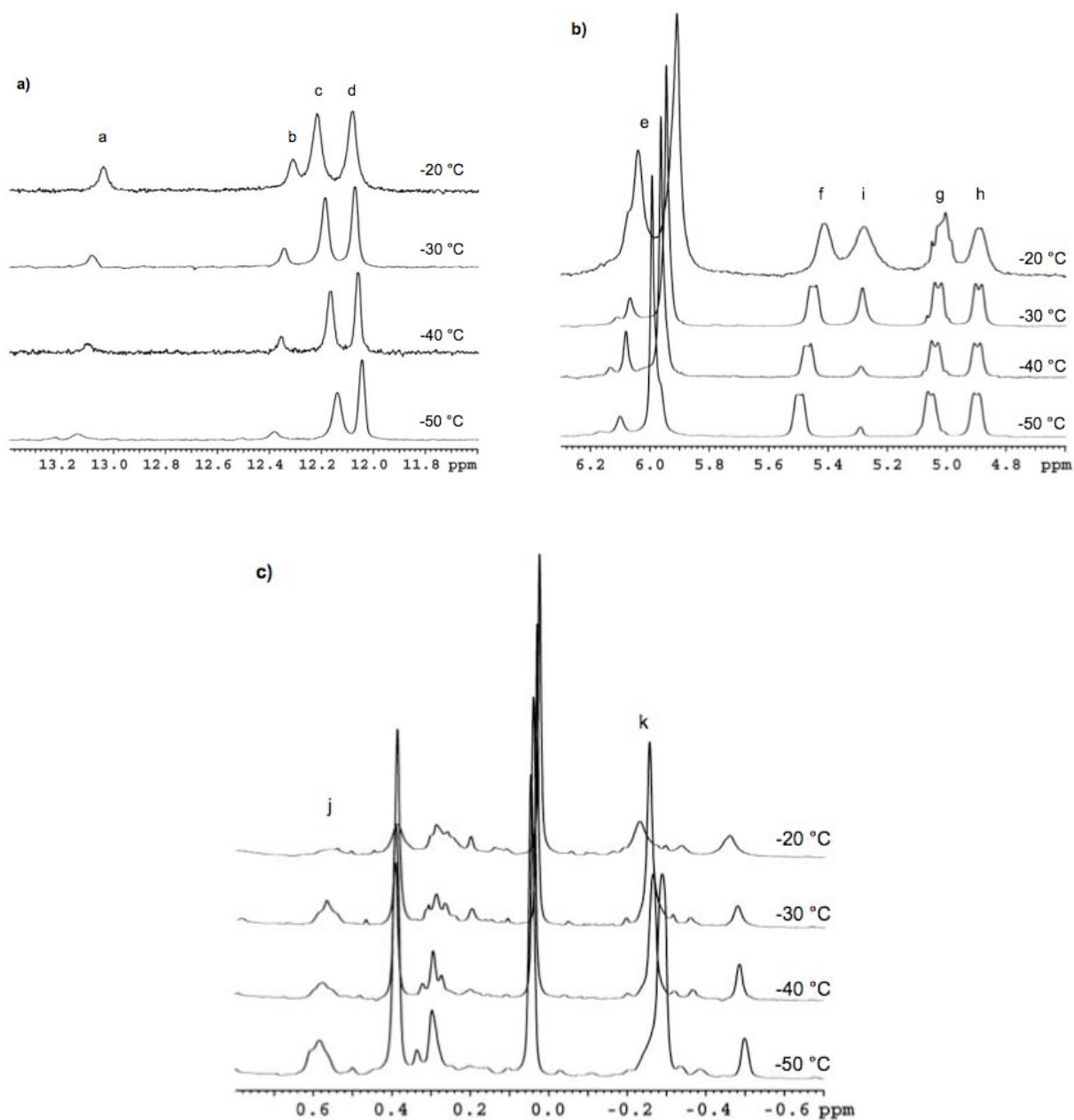
Figure 4. Proton NMR spectra of Mo(NAr)(C 3 H 6 )(OBitet)(Me 2 Pyr) ( 4 Mo ) in toluene-d 8 at -20 °C. (a) Expansion of the 1 H NMR spectrum in the alkylidene region for ( S )- and ( R )-Mo(NAr)(CH 2 )(Me 2 Pyr)(OBitet) (1 : 4 ratio of ( S )- 9 and ( R )- 9 ); (b) Expansion of the 1 H NMR spectrum in the H α region for Mo(NAr)(C 3 H 6 )(OBitet)(Me 2 Pyr) ( 4 Mo ). (c) Expansion of the 1 H NMR spectrum in the H β region for 4 Mo . (See Scheme 1 for labels.)
