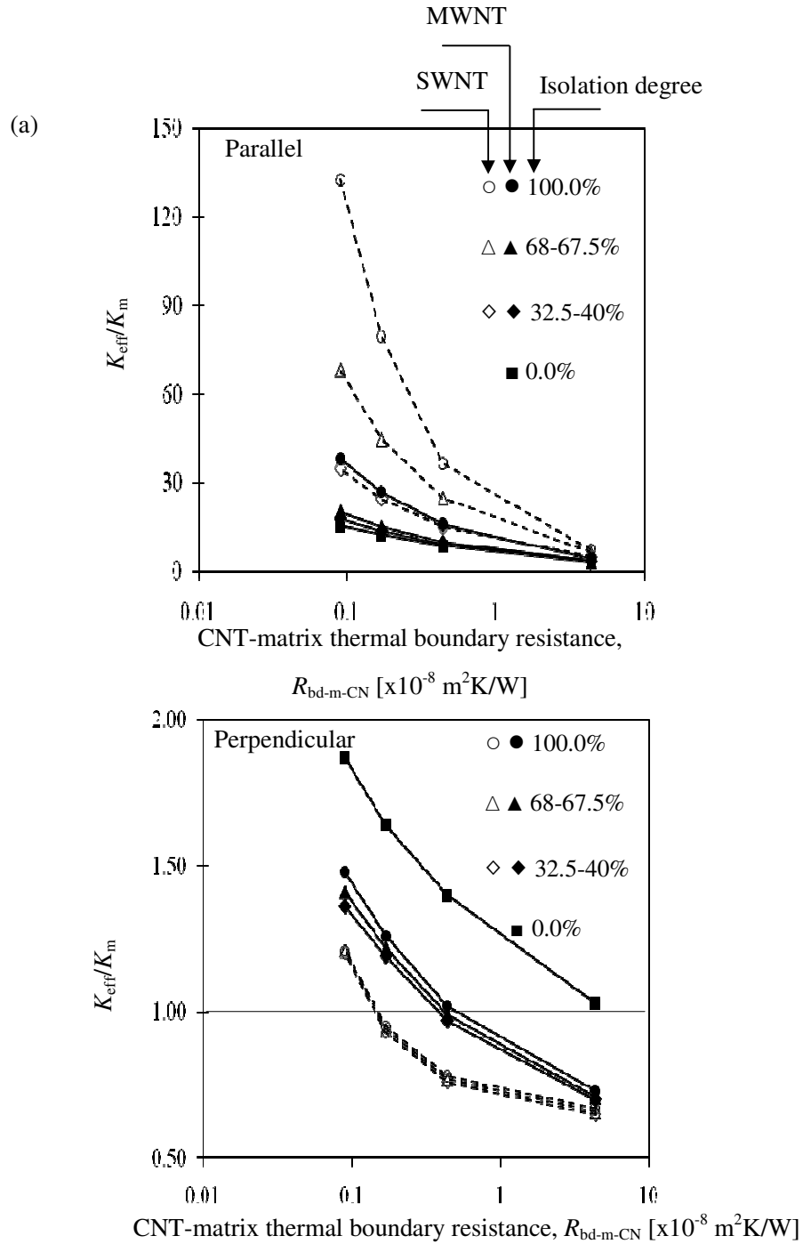
Figure 5. Comparison of effective thermal conductivity of MWNT-epoxy (solid dots and solid lines) and SWNT-epoxy (open dots and dashed lines) composites having 20vol% and highest CNT-CNT TBR, R_{bd-CN-CN} = 24.8 \times 10^{-8} m^2K/W as a function of CNT-matrix thermal boundary resistance with different CNT isolation degree and the CNTs oriented (a) parallel and (b) perpendicular to the heat flux.
