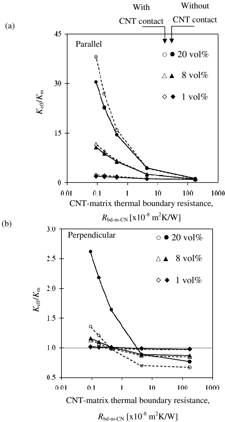
Figure 3. Comparison of effective thermal conductivity of MWNT-epoxy with (open dots, lowest CNT-CNT TBR, R_{\text{bd-CN-CN}} = 1.73 \times 10^{-8} \text{ m}^2\text{K/W} ) and without (solid dots) CNT-CNT contact as a function of CNT-matrix thermal boundary resistance with different volume fractions of CNTs and the CNTs oriented (a) parallel and (b) perpendicular to the heat flux.
