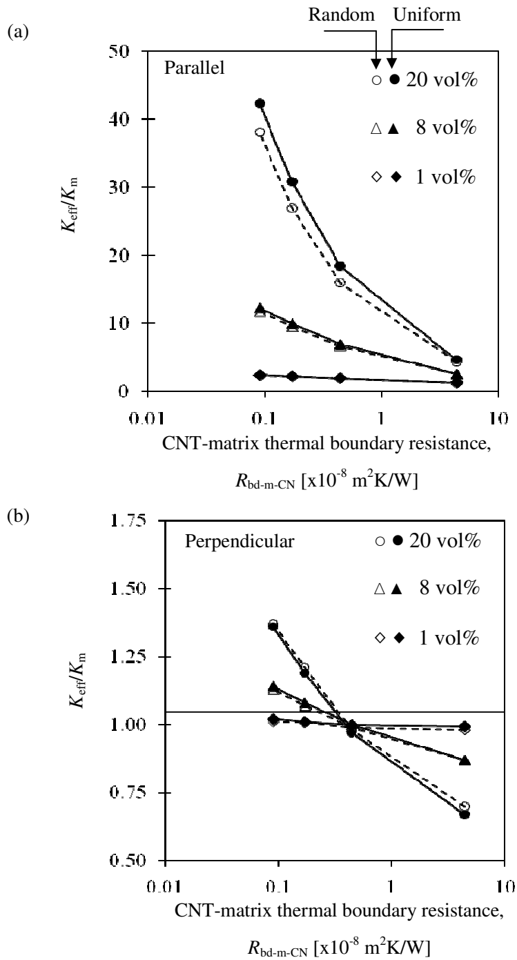
Figure 6. Comparison of effective thermal conductivity of MWNT-epoxy having no CNT-CNT contact with uniform CNT distribution (solid dots) and with random CNT distribution (open dots) effects as a function of CNT-matrix thermal boundary resistance with different volume fractions of CNTs and the CNTs oriented (a) parallel and (b) perpendicular to the heat flux.
