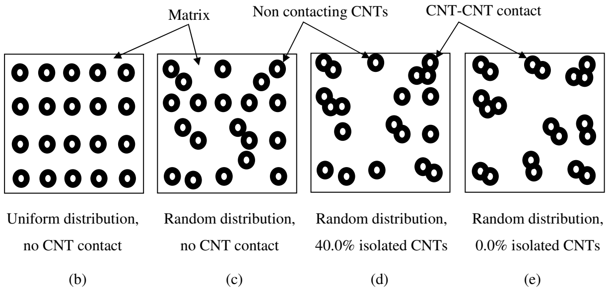
Figure 1. This figure is irrespective of SWNT and MWNT, it covers both. Parameters used in this study: (a) Schematic drawing of CNTs with different interfaces and therefore TBRs, and a top (y-z plane) view of 20 CNTs (b) uniform CNT distribution (square packing); (c) 100.0 % CNT isolation degree (no contact); (d) random distribution and random contact (40.0% isolated CNTs); and (e) random distribution with 0.0% isolated CNTs dispersed in the CNT-epoxy composite at 20 vol% of the CNTs, respectively.
