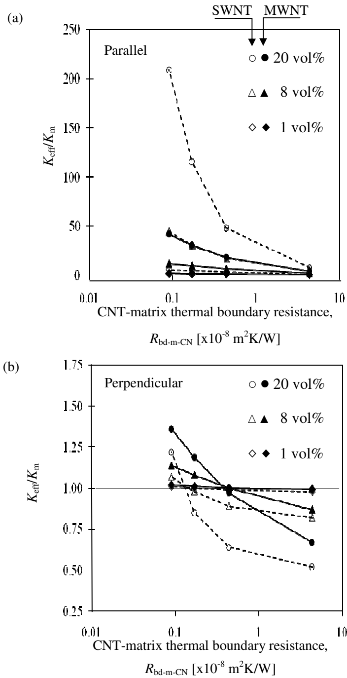
Figure 7. Comparison of effective thermal conductivity of MWNT-epoxy (solid dots, solid lines) and SWNT-epoxy (open dots and dashed lines) composites having no CNT-CNT contact with uniform CNT distribution as a function of CNT-matrix thermal boundary resistance with different volume fractions of CNTs and the CNTs oriented (a) parallel and (b) perpendicular to the heat flux.
