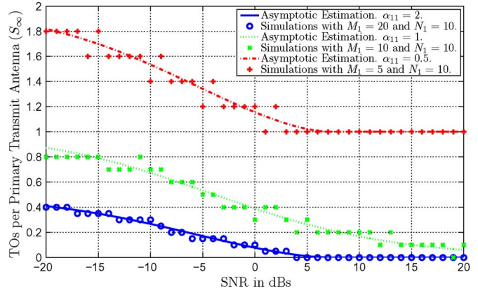
Fig. 2. Fraction of transmit opportunities in the RLNA (Def. 4), i.e., S_\infty (27) as function of the SNR = p_{1,\max}/\sigma_1^2 and \alpha_{11} = M_1/N_1 . Simulation results are obtained by using one realization of the matrix \mathbf{H}_{11} when N_1 = 10 .
