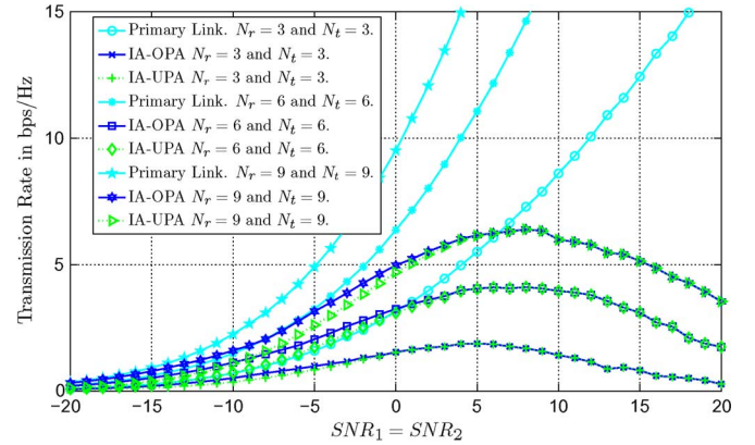
Fig. 4. Transmission rate of the opportunistic link obtained by Monte Carlo simulations as a function of the \text{SNR}_1 = \text{SNR}_2 . The number of antennas satisfy M_1 = M_2 = N_t and N_1 = N_2 = N_r , with N_t = N_r , and N_r \in \{3, 6, 9\} and \text{SNR}_i = p_{i,\max}/\sigma_i^2 , for all i \in \{1, 2\} .
