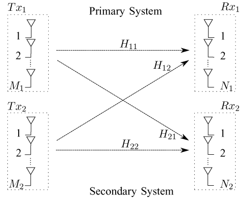
Fig. 1. Two-user MIMO interference channel.
