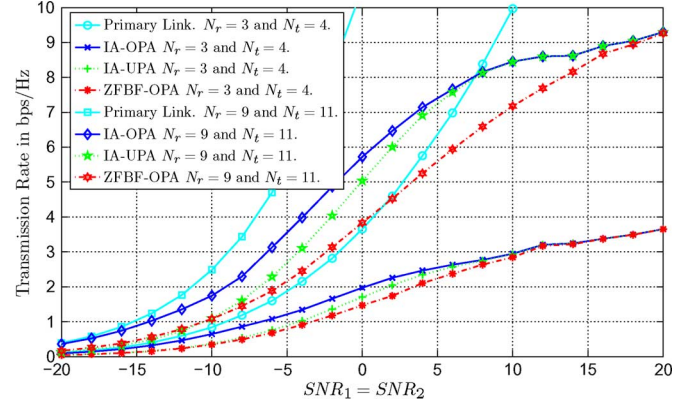
Fig. 3. Transmission rate of the opportunistic link obtained by Monte Carlo simulations as a function of the \text{SNR}_1 = \text{SNR}_2 when IA and ZFBF are implemented. The number of antennas satisfy \alpha = N_t/N_r \approx 5/4 , with M_1 = M_2 = N_t and N_1 = N_2 = N_r \in \{3, 9\} and \text{SNR}_i = p_{i,\max}/\sigma_i^2 , for all i \in \{1, 2\} .
