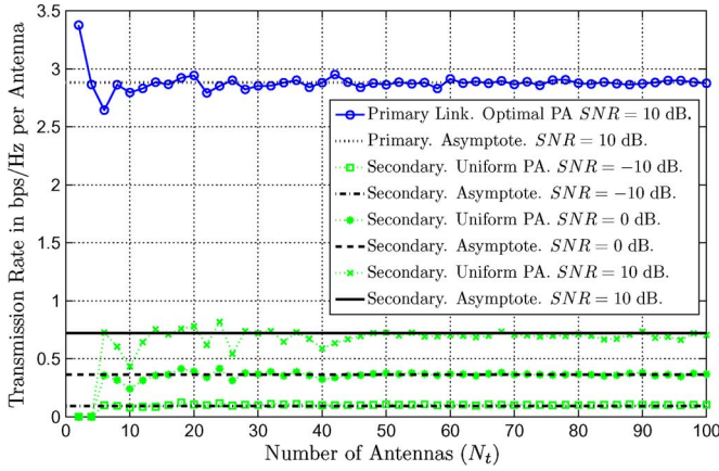
Fig. 6. Asymptotic transmission rates per antenna of the opportunistic link as a function of the number of antennas when N_r = N_t using uniform PA at different SNR levels \text{SNR}_i = p_{i,\max}/\sigma_i^2 . Simulation results are obtained using one channel realization for matrices \mathbf{H}_{ij} \forall (i, j) \in \{1, 2\}^2 and theoretical results using Proposition 5.
