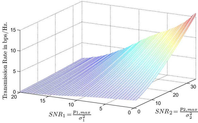
Fig. 5. Transmission rate of the opportunistic link obtained by Monte Carlo simulations as a function of the \text{SNR}_i = p_{i,\max}/\sigma_i^2 , with i \in \{1, 2\} . The number of antennas satisfy M_1 = M_2 = N_t and N_1 = N_2 = N_r , with N_r = N_t = 4 .
