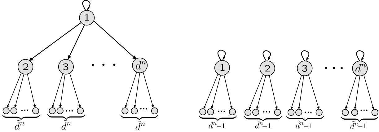
(a) \mathcal{E}_n : high degree sectors share a common supplier (b) \widehat{\mathcal{E}}_n : high degree sectors do not share a common supplier
