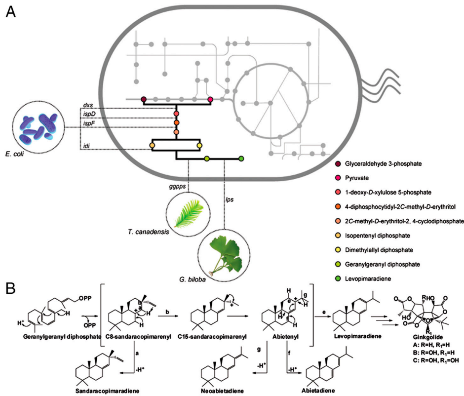
Fig. 1. (A) Engineering levopimaradiene synthesis in E. coli . A plant-derived pathway was constructed by introducing T. canadensis ggpps and G. biloba lps codon-optimized genes. To amplify the endogenous precursor pools of GGPPS substrates (IPP and DMAPP), copy numbers of rate-limiting steps ( dxs , idi , ispD , ispF ) in the MEP pathway were amplified by additional episomal expression. (B) General reaction mechanism of “LPS-type” enzymes. Levopimaradiene, the major product of G. biloba LPS is the gateway precursor of ginkgolides. Coproducts of LPS include abietadiene, neoabietadiene, and sandaracopimaradiene that stem from the different deprotonation patterns throughout intermediates in the reaction cascade.
