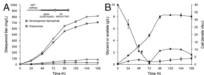
Fig. 5. Cultivation of the E. coli strain overexpressing the MEP pathway and the "reprogrammed" plant-derived pathway constituting GGPPS S239C/G295D and LPS M593I/Y700F mutants. (A) Diterpenoid production curves. Total diterpenoid, levopimaradiene, abietadiene, and sandaracopimaradiene are in circles, squares, triangles, and crosses, respectively. (B) Feed, fermentative by-product, and biomass curves. Glycerol, acetate, and cell density are in triangles, diamonds, and circles, respectively. Inverse triangle denotes the time point where 3 g of glycerol was added every 8 h.
