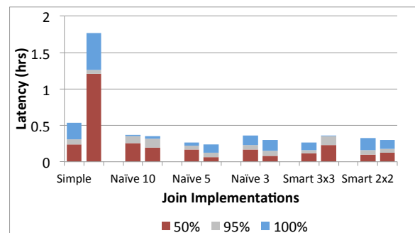
4: Completion time in hours of the 50 th , 95 th , and 100 th percentile assignment for variants of celebrity join on two tables with 30 celebrities each.
