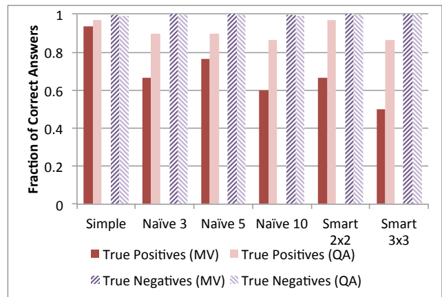
3: Fraction of correct answers on celebrity join for different batching approaches. Results reported for ten assignments aggregated from two runs of five assignments each. Joins are conducted on two tables with 30 celebrities each, resulting in 30 matches (1 per celebrity) and 870 non-matching join pairs.
