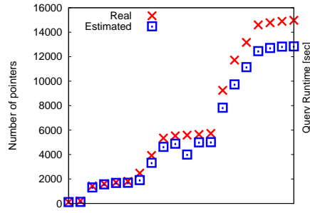
Figure 11: #Cutoff-Pointers Estimation
