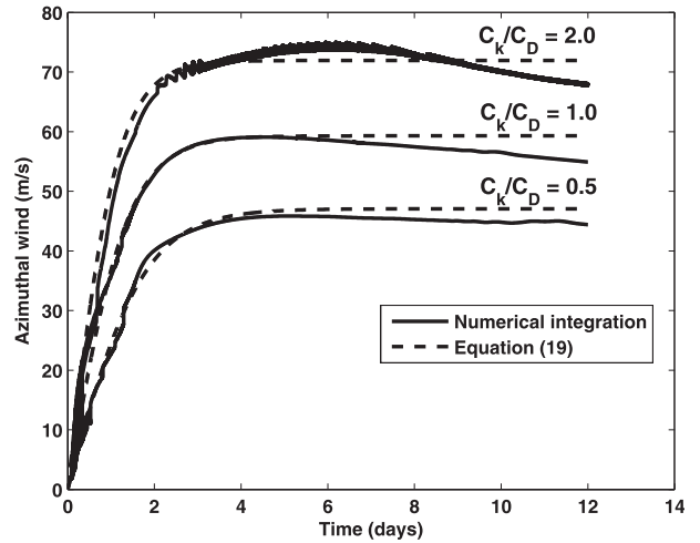
FIG. 1. Evolution with time of the peak azimuthal wind in the numerical simulations (solid) compared to the analytic approximation (19) (dashed) for three values of the ratio of exchange coefficients and with \alpha = 500 . In these simulations, the drag coefficient has been varied to control the variation of the ratio of exchange coefficients.
