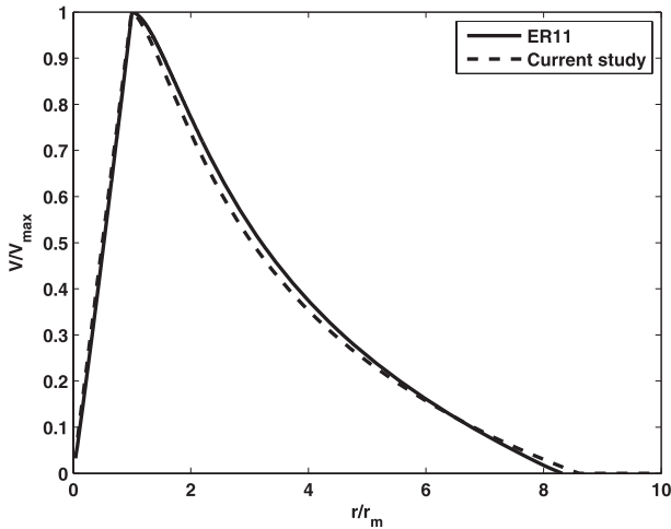
FIG. 2. Radial profile of azimuthal velocity from the steady-state model of Part I (solid) and at day 12 in the simulation using the time-dependent model (dashed); in both cases C_r = 1 . The radius has been normalized by the radius of maximum winds and the azimuthal wind has been normalized by its maximum value.
