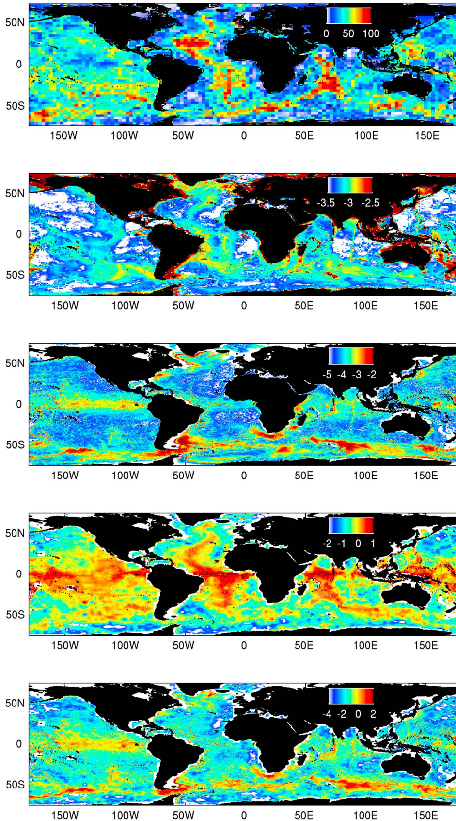
Figure 2. (top) Topographic roughness in (m). (middle top) Bottom stratification in \log_{10} (\text{s}^{-1}) estimated using the WOCE hydrographic atlas. (middle) Bottom kinetic energy in \log_{10} (\text{m}^2 \text{s}^{-2}) obtained from the isopycnal ocean model. (middle bottom) Topographic steepness parameter, \log_{10} \epsilon . (bottom) Energy flux into internal lee waves in \log_{10} (\text{mW m}^{-2}) .
