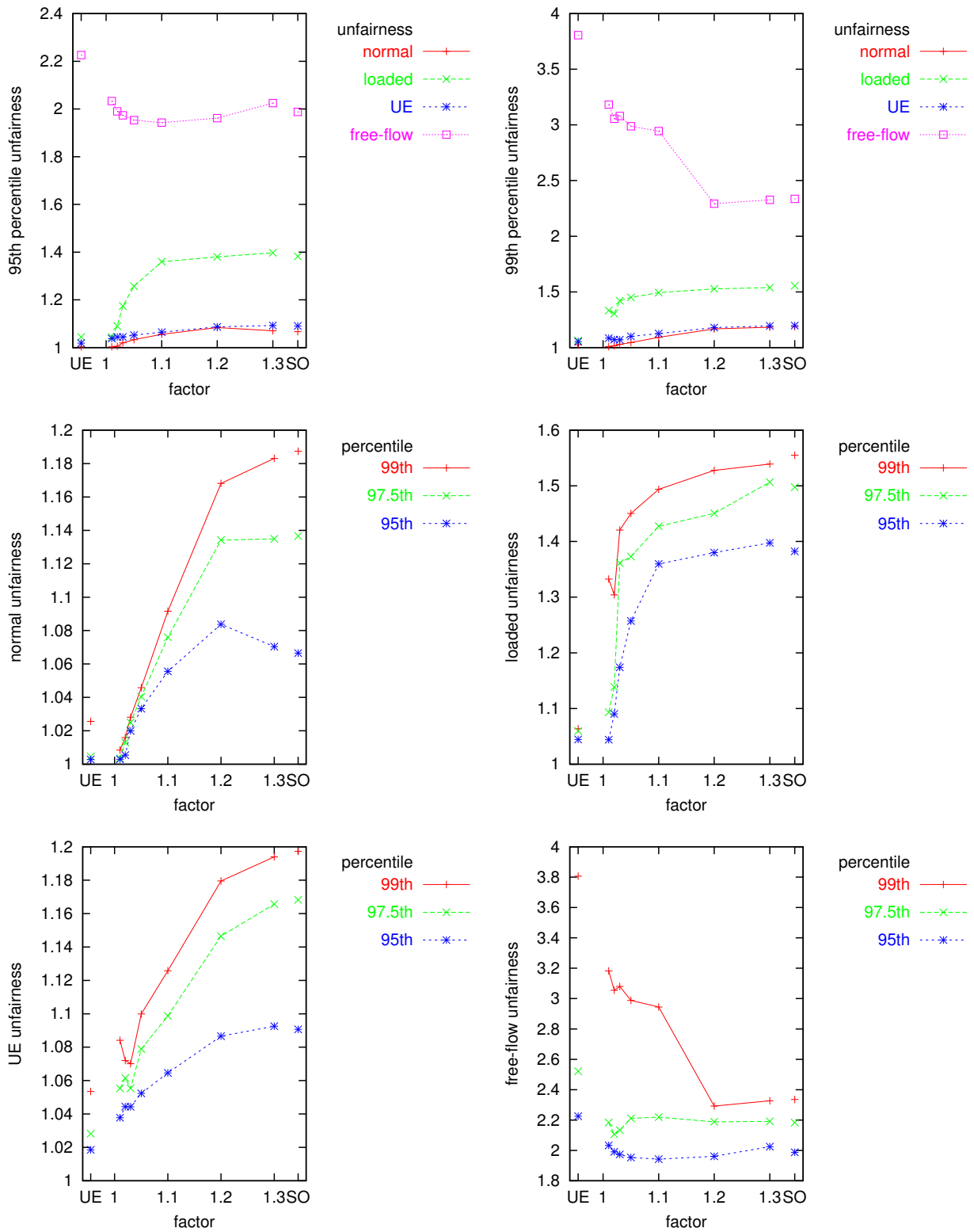
FIGURE 11. Unfairness over the different factors and percentiles for instance Neukölln
