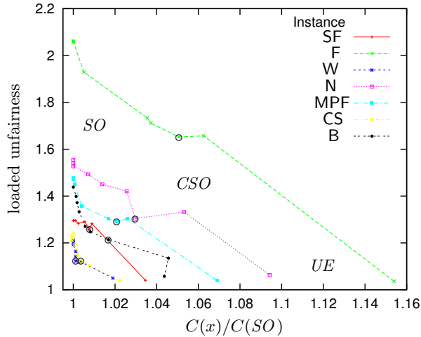
FIGURE 15. Tradeoff between efficiency and unfairness. For all instances, we plot the tradeoff curve between the efficiency (the cost of the solution over the cost of the system optimum) vs. the loaded unfairness. The left area of the graph corresponds to system optima (SO), the lower area corresponds to user equilibria (UE), and the circled data-points (denoted with ‘o’) correspond to constrained system optima with \varphi = 1.02 ( CSO^{1.02} ).
