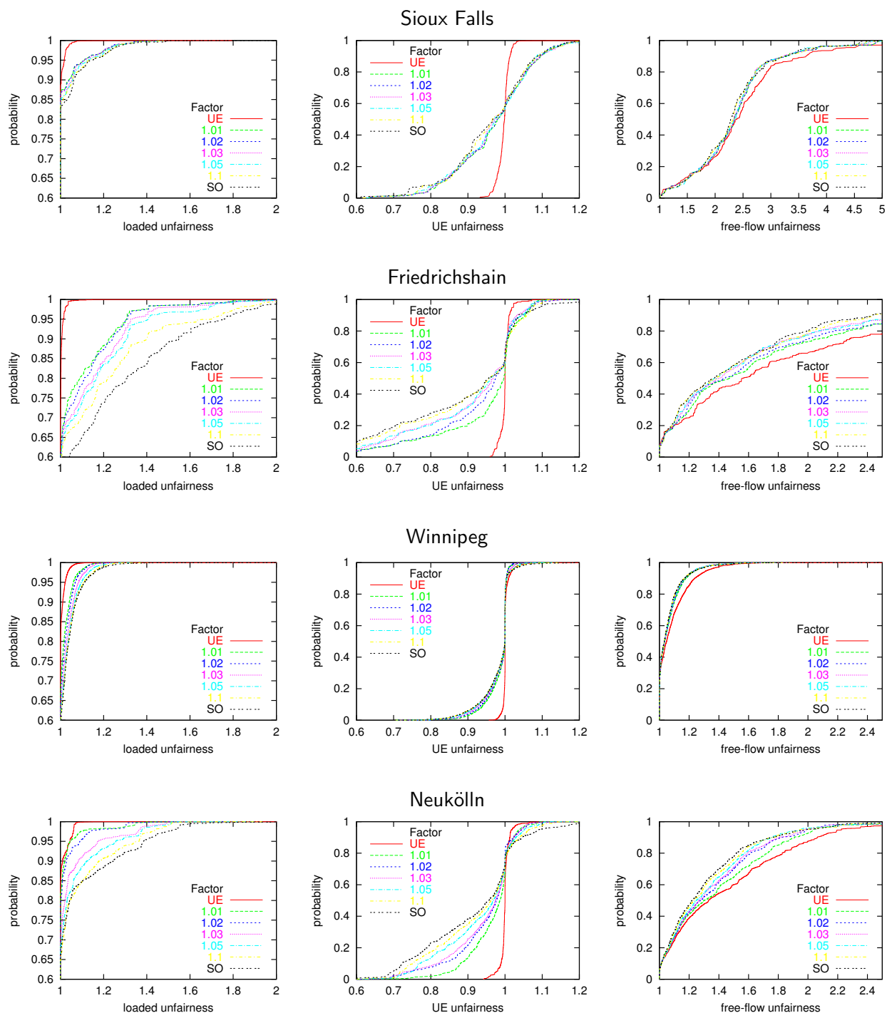
FIGURE 5. Unfairness distributions for various tolerance factors, Part I
