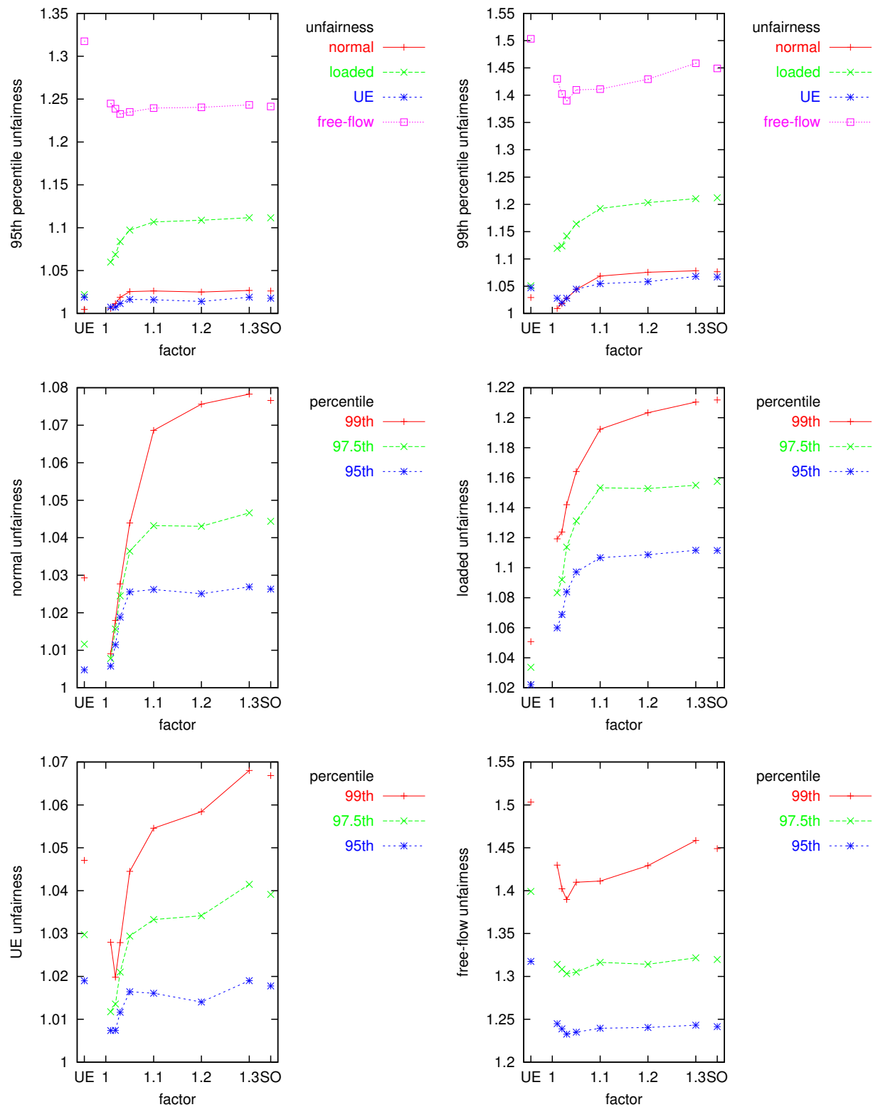
FIGURE 9. Unfairness over the different factors and percentiles for instance Winnipeg
