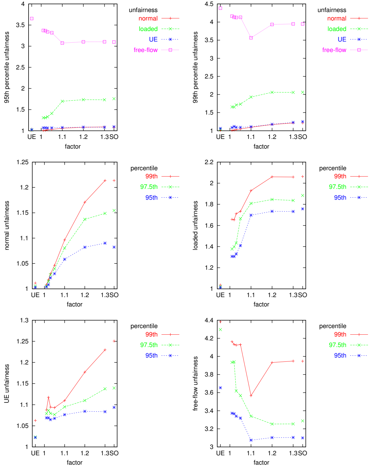
FIGURE 8. Unfairness over the different factors and percentiles for instance Friedrichshain
