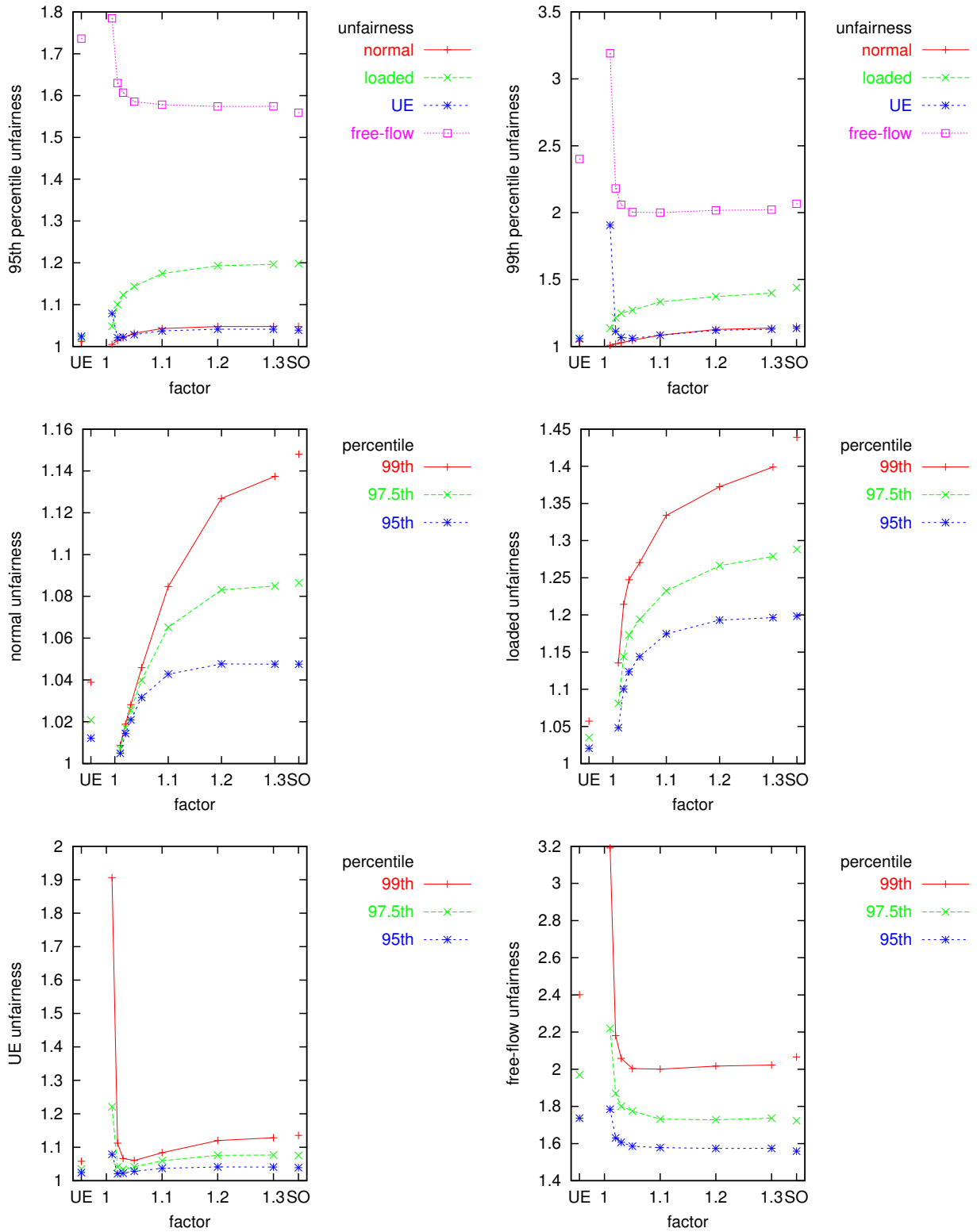
FIGURE 13. Unfairness over the different factors and percentiles for instance Berlin
