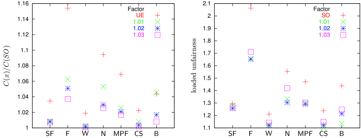
FIGURE 14. Efficiency and loaded unfairness of constrained system optima across all instances. The plot on the left shows the efficiency (the cost of the solution over the cost of the system optimum) of select constrained system optima vs. that of the associated user equilibria; the plot on the right compares the loaded unfairness of the same solutions with that of the corresponding system optima.
