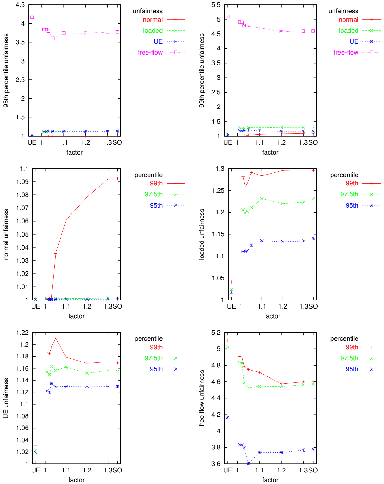
FIGURE 7. Unfairness over the different factors and percentiles for instance Sioux Falls
