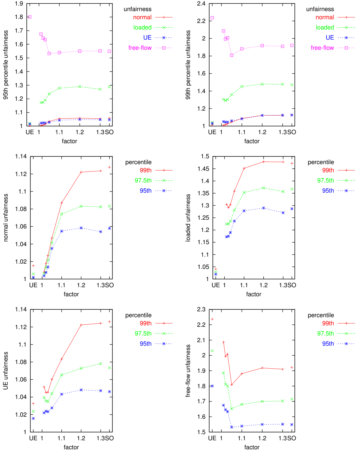
FIGURE 10. Unfairness over the different factors and percentiles for instance ‘Mitte, Prenzlauerberg & Friedrichshain’
