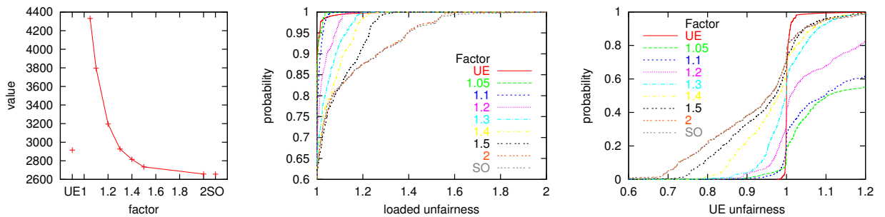
FIGURE 3. Objective values and unfairness distributions for instance Neukölln and normal lengths equal to free-flow travel times
