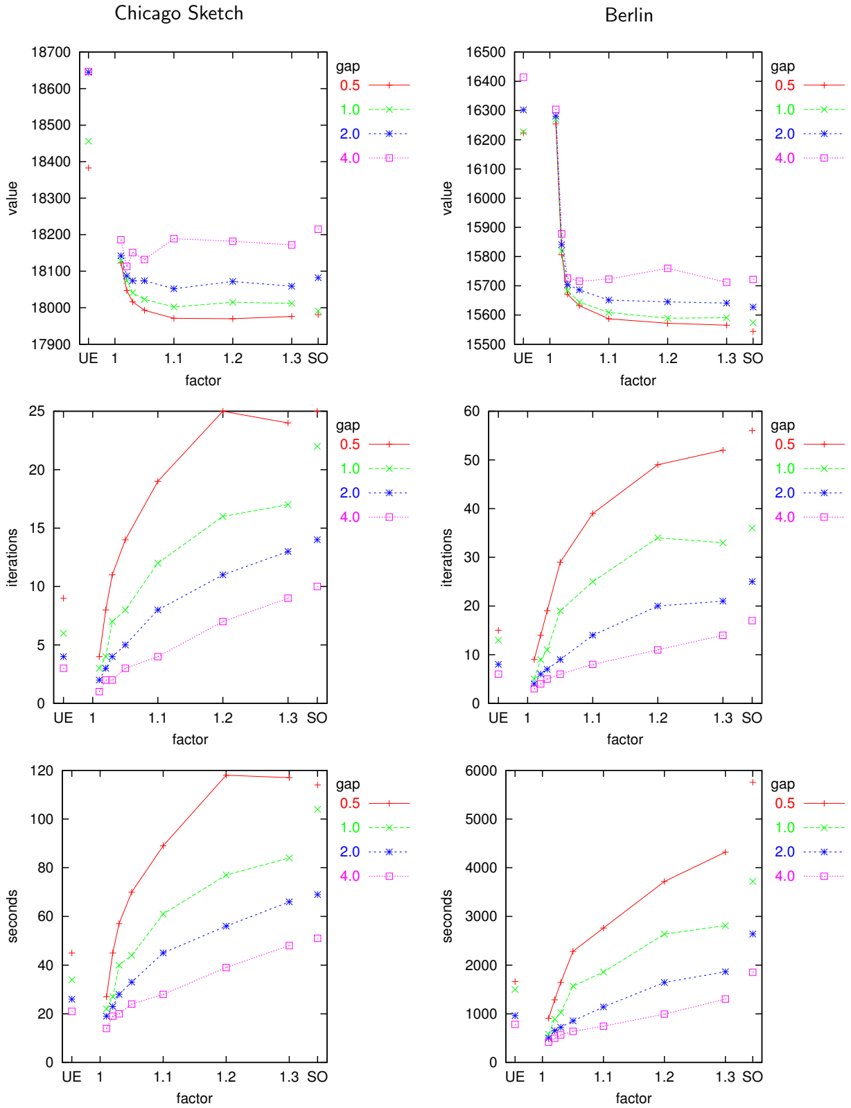
FIGURE 16. Specifics of the algorithm for various optimality gaps and tolerance factors for instances Chicago Sketch and Berlin
