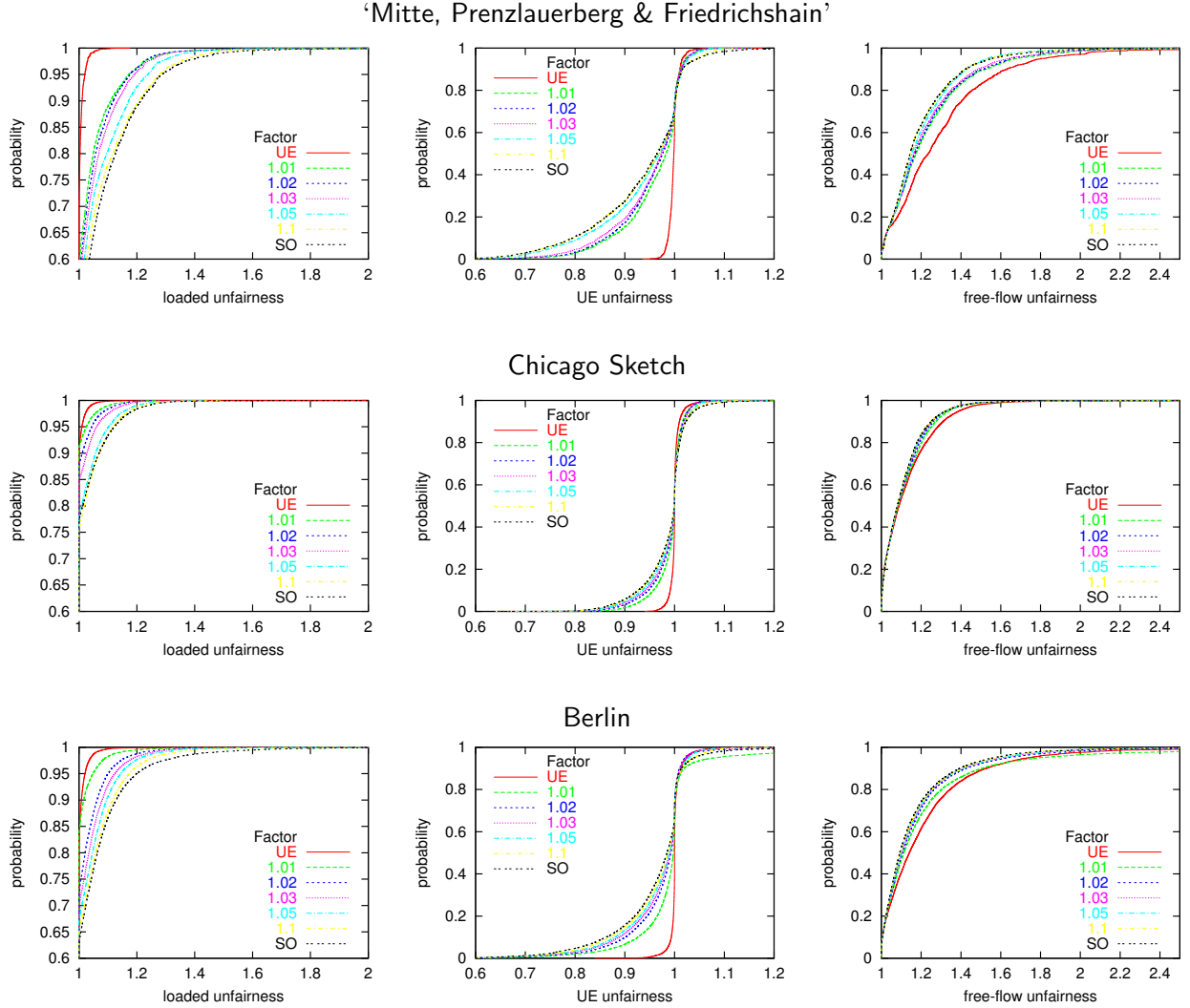
FIGURE 6. Unfairness distributions for various tolerance factors, Part II
