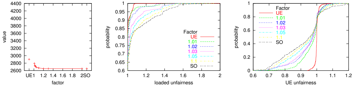
FIGURE 4. Objective values and unfairness distributions for instance Neukölln and normal lengths equal to travel times in user equilibrium
