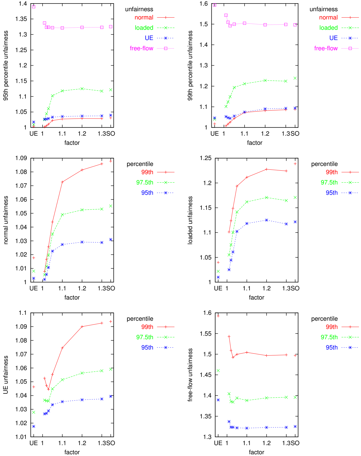
FIGURE 12. Unfairness over the different factors and percentiles for instance Chicago Sketch
