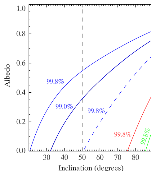
Figure 2. Inclinations and albedos for which an atmosphere can be inferred. Each line is the locus of orbit inclination and albedo values that would produce an 8 \mu\text{m} sinusoidal flux modulation corresponding to our 99.8% and 99.0% confidence upper limits ( 44 & 34 \mu\text{Jy} ). Color encodes planet composition: pure water ice planets (solid blue curve); "dirty" ocean planets (dashed blue curve, 6.5% by mass iron core, 48.5% silicate mantle, and 45% ice outer layers, or different combinations with the same mass and radius); an Earth-like composition (red curve, 32.5% iron core and 67.5% silicate mantle); and a Mercury-like composition (green curve, 70% iron core and 30% silicate mantle). A GJ 876 with no atmosphere is allowed by our data above each line; the regions below the line are forbidden at that confidence level. In other words, if GJ 876d has a composition, orbit inclination, and albedo lying in the regions below the curves, then we would infer the presence of an atmosphere.
