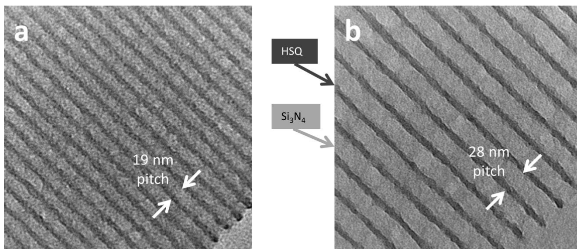
Figure 2. Transmission electron micrographs of developed gratings written into 16-nm-thick HSQ on a 50-nm-thick \text{Si}_3\text{N}_4 membrane using 20 keV \text{Ne}^+ . (a) 19-nm-pitch gratings written using a linear dose of 22 ions/nm. (b) 28-nm-pitch gratings written using a linear dose of 19 ions/nm. In (a), the unpatterned region of the lower right corner is lighter than the regions between lines; this thickness contrast indicates the presence of resist residues. Such residues are not apparent in (b). Thus, the contrast of developed structures depends on pattern density.
