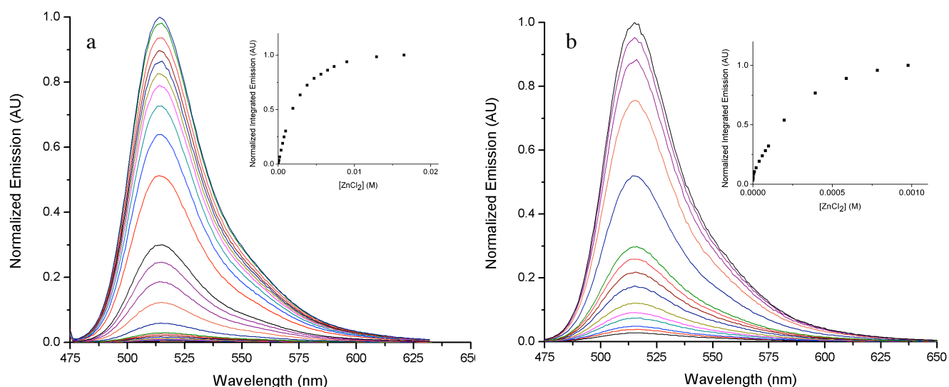
Figure 2. Normalized fluorescence response in the presence of excess \text{ZnCl}_2 of a) 1 \mu\text{M} QZ2E, 0 - 20 \text{ mM} \text{ZnCl}_2 and b) 1 \mu\text{M} QZ2A, 0 - 1 \text{ mM} \text{ZnCl}_2 in 50 \text{ mM} PIPES, 100 \text{ mM} KCl, \text{pH } 7.0 , T = 25 \text{ }^\circ\text{C} . Insets: Integrated fluorescence vs. \text{ZnCl}_2 concentration, normalized and adjusted for the basal fluorescence of the sensor in the absence of \text{Zn(II)} .
