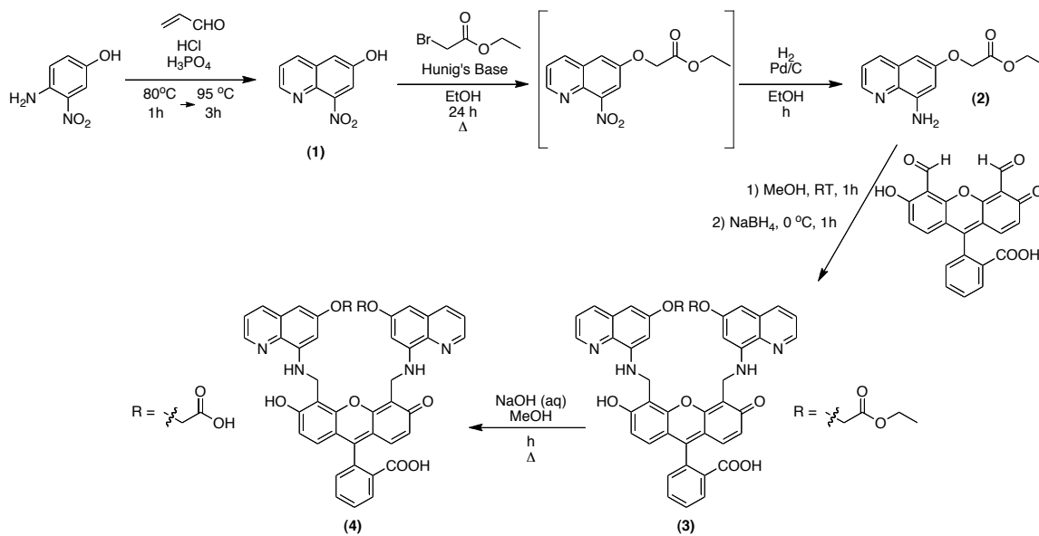
Scheme 1. Syntheses of QZ2E and QZ2A.
