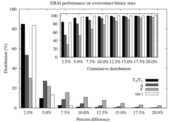
Figure 9. Distributions of differences between the test set and the network output for overcontact binaries. The inset depicts the cumulative distributions. While the inclination and the temperature ratio are remarkably well determined, the mass ratio is determined reliably only for high inclination systems, and fillout factor is quite dispersed. Nevertheless, 90% of all systems have errors in all four parameters smaller than 15%.
