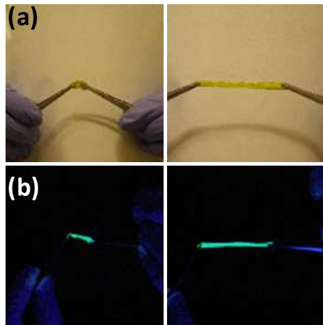
Figure 3. (a) Optical micrographs of PNB crosslinked with P1 in unstretched (left) and stretched (right) states. (b) Optical micrographs with 365 nm excitation light of the same material in unstretched (left) and stretched (right) states.
