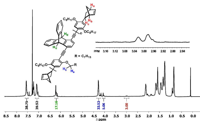
Figure 1. ^1\text{H} NMR spectrum of polymer P2 . Included is the molecular structure of P2 with appropriate protons highlighted as well as a magnified region of the spectrum as an inset.
