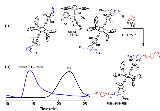
Figure 2. (a) Synthesis of PNB-b-P1-b-PNB . (b) THF SEC (UV detection 450 nm) traces of P1 (black) and PNB-b-P1-b-PNB triblock copolymer (blue).
