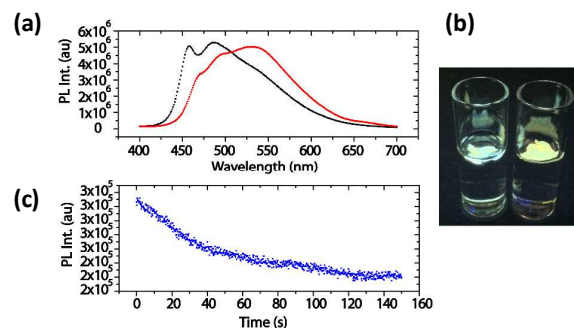
Figure 4. (a) Photoluminescence spectra of PNB crosslinked with P2 in water (red) and 1% THF:water (v:v) (black). (b) Optical micrograph (UV excitation at 365 nm) showing PNB crosslinked with P2 films in water (right) and 1% THF:water (v:v) (left). (c) Photoluminescence intensity decay (monitored at 450 nm) of the same film after exposure to the saturated vapor of THF.
