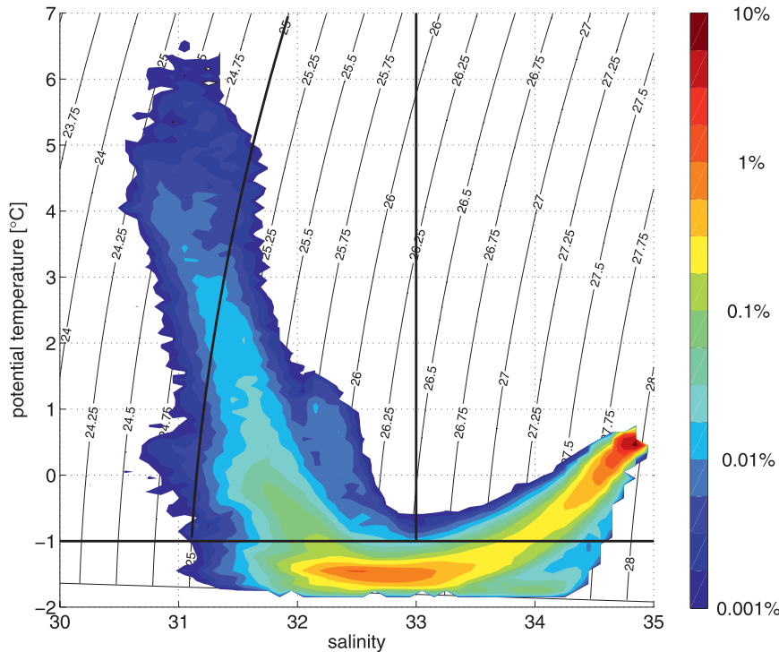
FIG. 4. Occurrence of water types as a function of temperature and salinity over the 2-yr deployment. Units are percentage of all measurements per 0.1^{\circ}\text{C} and 0.1 salinity (note the logarithmic scale). The 33 line separating the Pacific from the Atlantic Water and the -1^{\circ}\text{C} line separating the winter water are indicated along with the 25 \text{ kg m}^{-3} line separating the two summer water types.
