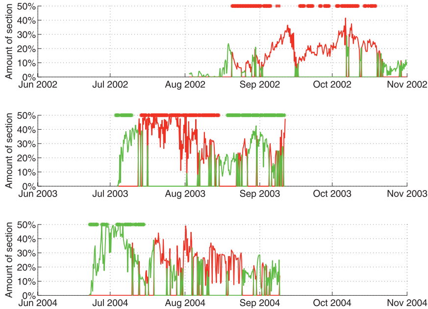
FIG. 6. Amount of area within the gray box of Fig. 2 occupied by ACW (red curve) and CSW (green curve) as a function of time. The time periods that have been considered for the composite averages of the boundary current are indicated by the symbols at the top of each row: ACW (red) and CSW (green). The record termination on 10 Sep 2003 is due to the mooring turnaround that lasted until 1 Oct 2003.
