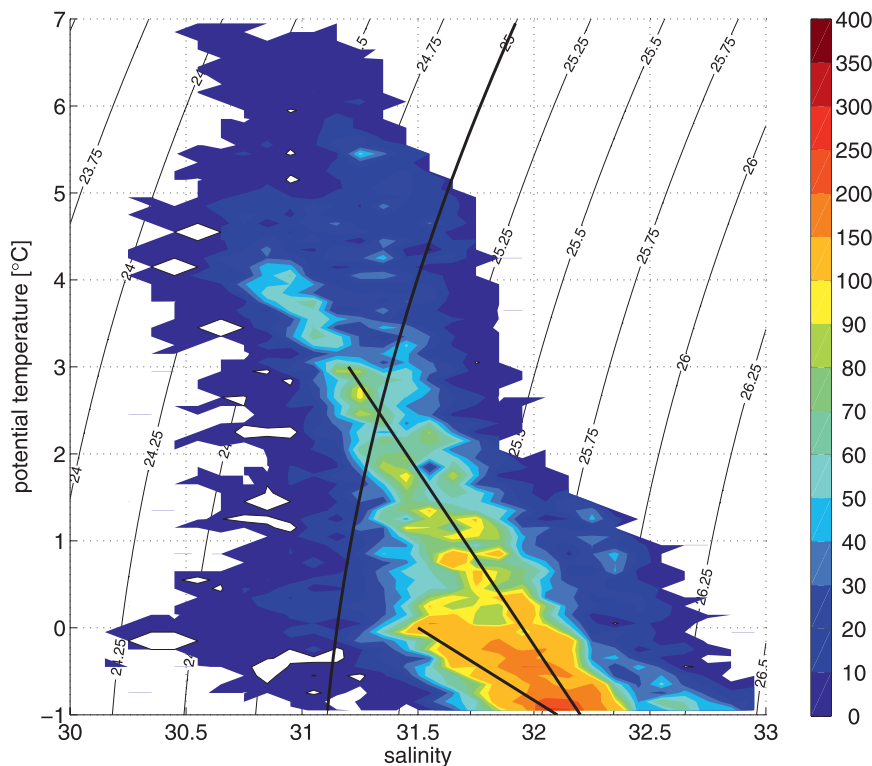
FIG. 5. Transport within the summer water domain ( S < 33 and \theta > -1^\circ\text{C} ) over the 2-yr deployment as a function of temperature and salinity. Units are \text{m}^3 \text{s}^{-1} per 0.1^\circ\text{C} and 0.1 salinity (note the nonlinear scale). The 25 \text{ kg m}^{-3} line separating the two summer water types is highlighted along with the major mixing lines between PWW and ACW and between PWW and CSW.
