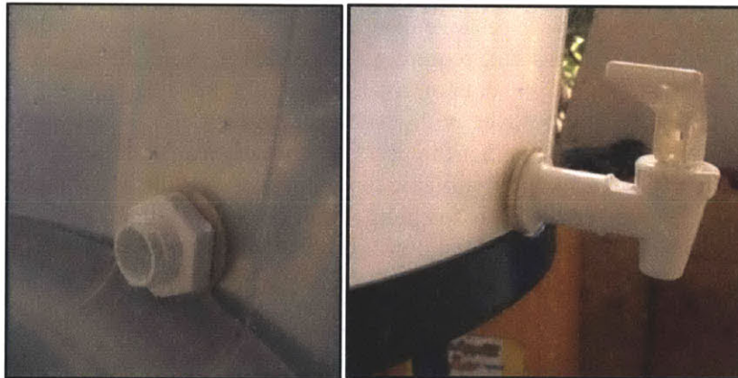
Figure 6-4: Left, Jam nut and washer, which attach the Tomlinson Industries spigot to the inside of the Kosim safe storage container; Right, Tomlinson Industries spigot and washer attached to the outside of the Kosim safe storage container.
