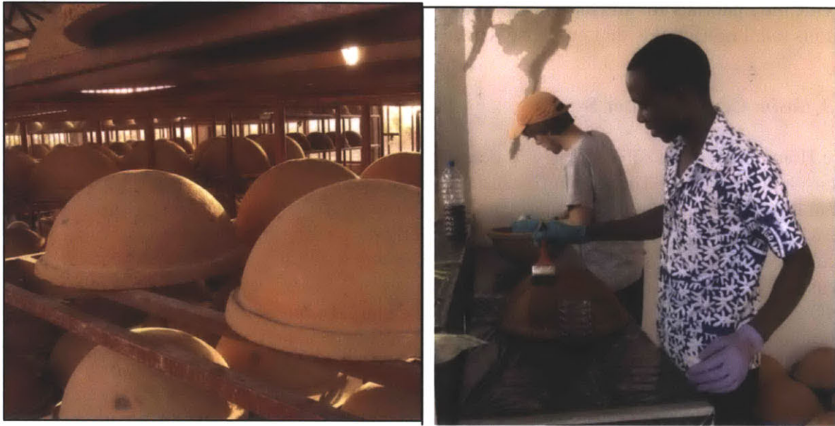
Figure 1-2: Left, Hemispheric ceramic water filters on cooling racks after firing process at PHW; Right, PHW employee and MIT graduate student painting filters with colloidal silver solution
