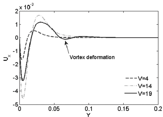
FIG. 7. Tangential velocity across a seed vortex at different bias voltages in the Ohmic ( V = 4 ) and limiting regimes ( V = 14 and 19 ). Action of an electric field on the extended space charge layer causes a deformation of seed vortices. The deformation is only significant at high bias voltages in the limiting-current regime (e.g., V = 19 ).
