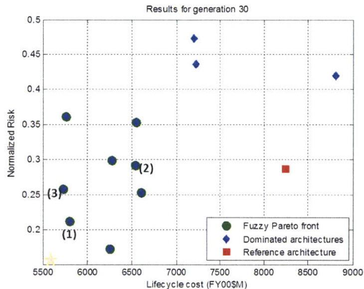
Figure 77: Iso-science, cost-risk space in the Decadal packaging problem
