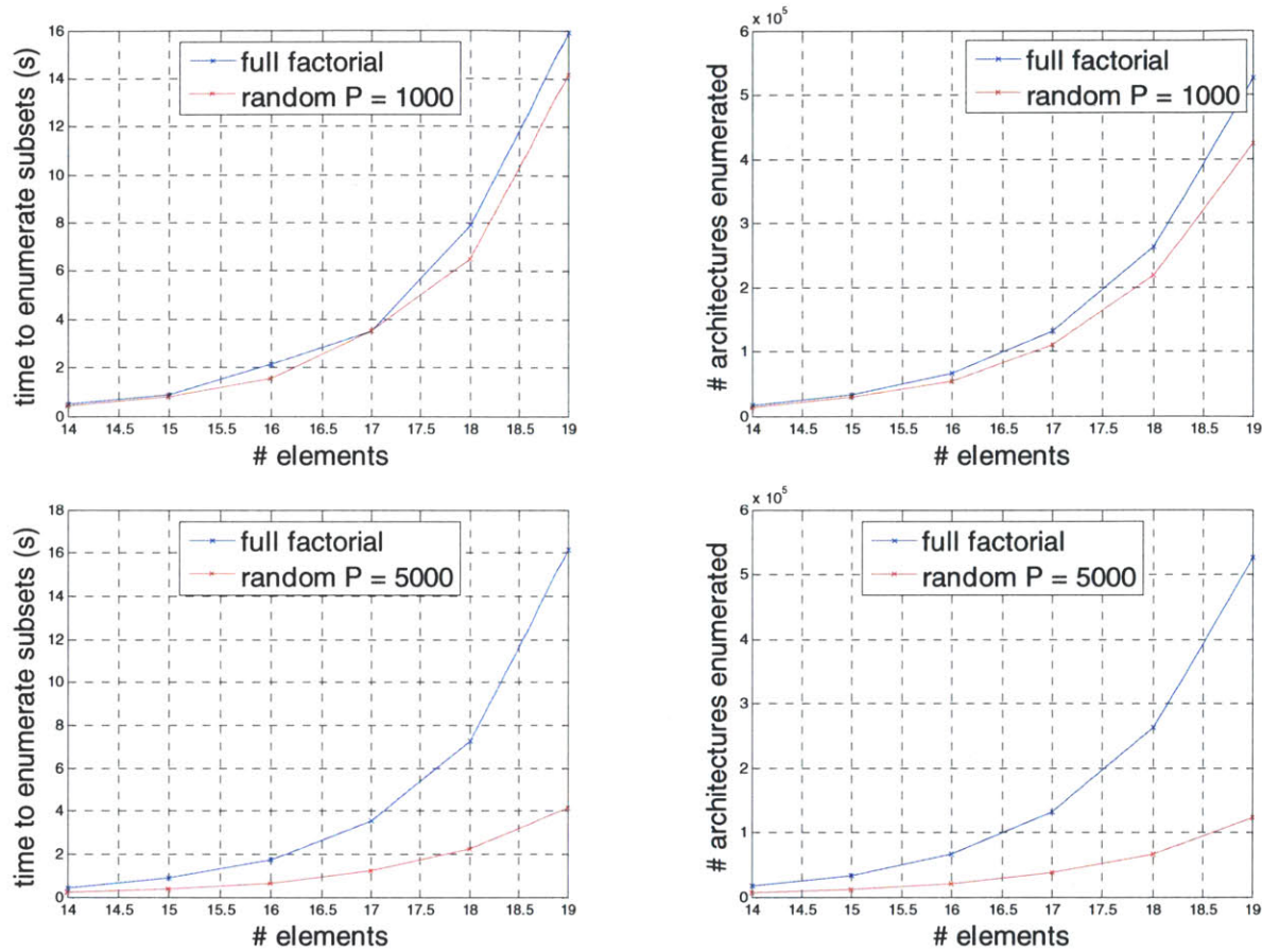
Figure 20: Performance of the two grammars proposed for the DsP for two different values of P
