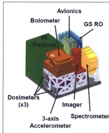
Figure 92: Preliminary allocation of system sensors and hosted payload on GeoSCAN
