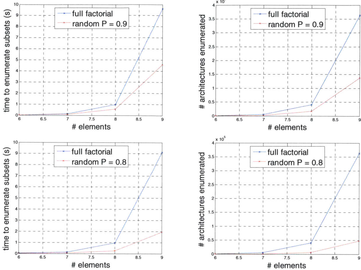
Figure 21: Performance of the two grammars for the PeP
