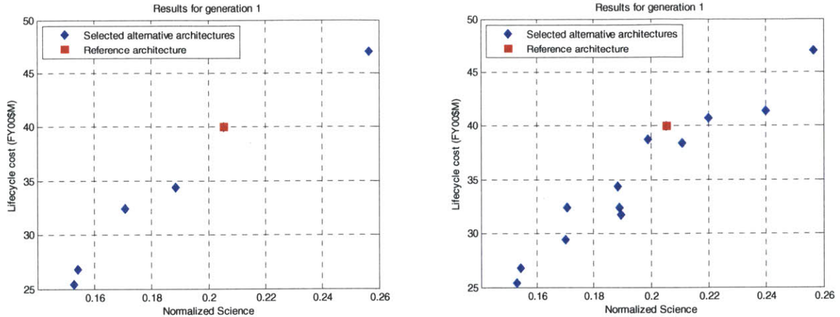
Figure 93: Fuzzy Pareto frontier of GeoSCAN selection architectures for two max levels of programmatic risk: 15% (left) and 30% (right)
