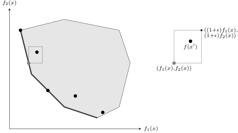
Figure 1: Figure illustrating the concept of Pareto-optimal front (shown by the thick boundary) and approximate Pareto-optimal front (shown by solid black points) for two objectives.
