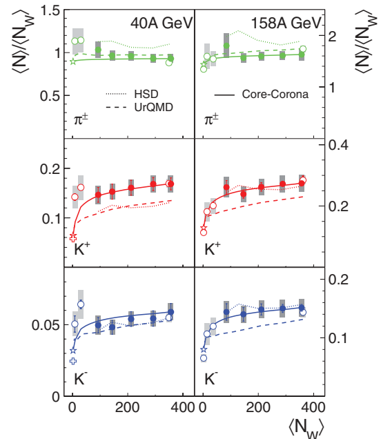
FIG. 10. (Color online) Particle yields divided by the mean number of wounded nucleons as a function of centrality. Closed symbols show results from centrality selected Pb + Pb collisions; open circles show p + p data from NA49 [9,10] as well as C + C , Si + Si (at 158A GeV [8]), and central Pb + Pb collisions from [2,3]. The stars denote the values obtained for p + p interactions from parametrization “B” in Ref. [38]. At 40 GeV/c the yields of K^\pm in p + p are compared to values extracted from Fig. 132 reported in [10] (open crosses). Lines show results from HSD [36] and UrQMD2.3 [37] calculations as well as from the core-corona model (the latter for the Pb + Pb collision system only [39]). The thin vertical bars indicate the statistical errors, which are mostly not visible. The thick shaded bars indicate the systematic errors.
