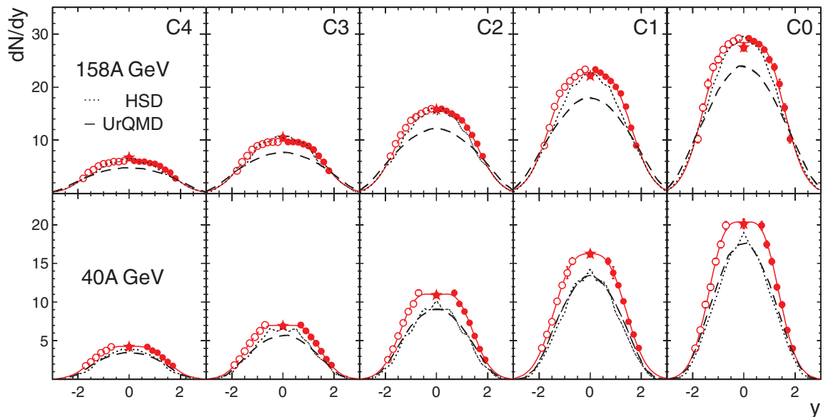
FIG. 6. (Color online) Rapidity spectra of K^+ in Pb + Pb collisions at 40A GeV and 158A GeV beam energy for different centrality bins labeled C0–C4. Circles are values from the dE/dx analysis; the stars give the results from the combined dE/dx and TOF analyses. Open symbols are reflected at mid-rapidity. Solid lines represent the fits of Eq. (2) (often not visible due to symbol size). The dotted and dashed lines represent HSD [36] and UrQMD2.3 [37] simulations, respectively. The error bars (mostly not visible) indicate the statistical uncertainty.
