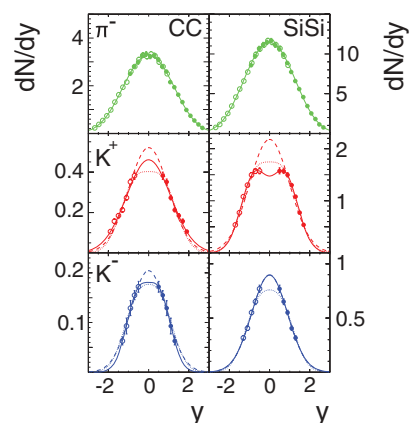
FIG. 8. (Color online) Rapidity spectra for \pi^- and K^\pm for semicentral C + C and Si + Si collisions at 40A GeV beam energy. Solid lines show free fits of double Gaussians. Open symbols are reflected at mid-rapidity. For K^\pm also double Gaussians with width \sigma and shift y_0 as for central Pb + Pb collisions at 40A GeV beam energy were fitted (short dashed line) as well as a single Gaussian with the same RM_S (dashed line). The error bars indicate the statistical uncertainty.
