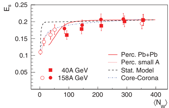
FIG. 14. (Color online) Total relative strangeness approximated by E_S for centrality selected minimum-bias Pb + Pb collisions at 40A GeV (squares) and 158A GeV (circles) as a function of \langle N_W \rangle . The open symbols are from p + p [9,10], C + C, Si + Si [2], S+S [40], and central Pb + Pb [2] at 158A GeV. The filled symbols represent the data of centrality selected Pb + Pb collisions at 40A GeV and 158A GeV (this analysis and [6]). The lines indicate calculations within the statistical model under the assumption of proportionality between ensemble volume and \langle N_W \rangle (dashed), with volumes as derived from percolation calculations for small systems (dotted line) and Pb + Pb collisions (solid line) [21], as well as calculations based on the core-corona ansatz at 158A GeV (dash-dotted line). Only statistical errors are shown.
