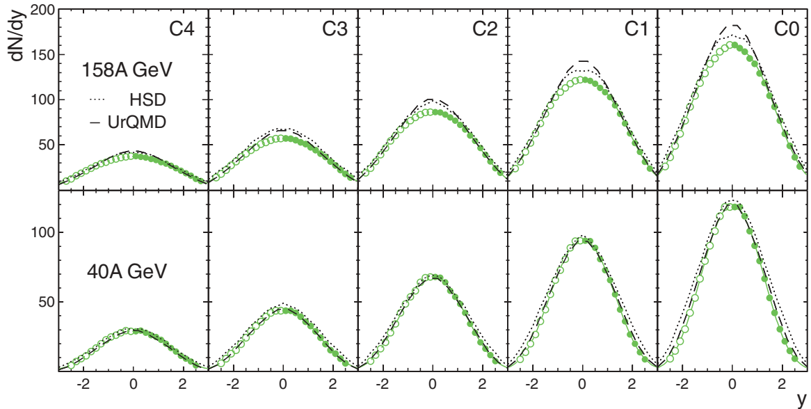
FIG. 5. (Color online) Rapidity spectra for \pi^- in Pb + Pb collisions at 40A GeV and 158A GeV beam energy for different centrality bins labeled C0–C4. Open symbols are reflected at mid-rapidity. Solid lines represent the fits of Eq. (2) (often not visible due to symbol size). The dotted and dashed lines represent HSD [36] and UrQMD2.3 [37] simulations, respectively. The error bars (mostly not visible) indicate the statistical uncertainty.
