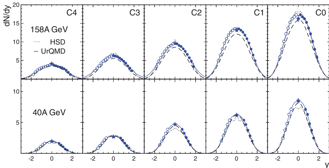
FIG. 7. (Color online) Rapidity spectra of K^- in Pb + Pb collisions at 40A GeV and 158A GeV beam energy for different centrality selections labeled C0–C4. Circles are values from the dE/dx analysis; the stars give the results from the combined dE/dx and TOF analysis. Open symbols are reflected at mid-rapidity. Solid lines represent the fits of Eq. (2). The dotted and dashed lines represent HSD [36] and UrQMD2.3 [37] simulations, respectively. The error bars (mostly not visible) indicate the statistical uncertainty.
