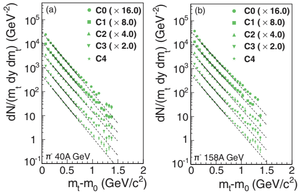
FIG. 2. (Color online) Transverse mass spectra at mid-rapidity ( 0 < y < 0.2 ) for \pi^- in Pb+Pb collisions at 40A GeV and 158A GeV beam energy. Lines show exponential fits for 0.2 < m_T - m_0 < 0.7 GeV/ c^2 . Different centralities are scaled for clarity. The error bars indicate the statistical uncertainty.
