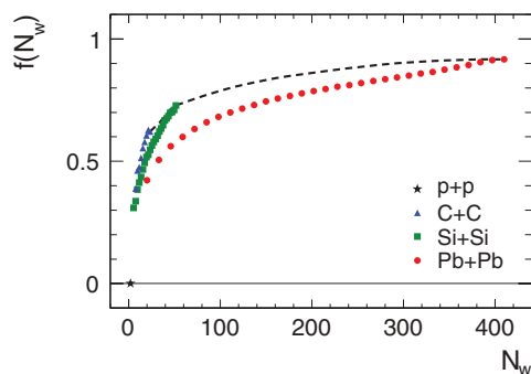
FIG. 12. (Color online) Core fraction obtained in the core-corona model for different collision systems as a function of the number of participating nucleons [39]. The dashed line connects the endpoints of the curves for the different collision systems. f(N_W) denotes the fraction of those nucleons which undergo more than one collision.
