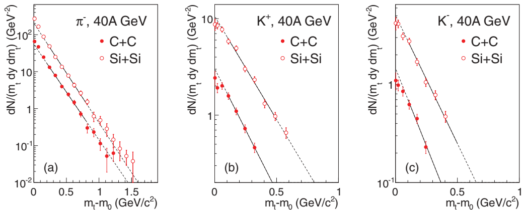
FIG. 3. (Color online) Transverse mass spectra of \pi^- ( 0 < y < 0.2 ) and kaons ( 0.8 < y < 1.0 ) at 40A GeV in C + C and Si + Si collisions. Lines show exponential fits for 0.2 GeV/ c^2 < m_T - m_0 < 0.8 GeV/ c^2 ( \pi^- ) and 0.1 GeV/ c^2 < m_T - m_0 < 0.5 GeV/ c^2 (kaons). The inverse slope parameters for K^+ ( K^- ) are 171 \pm 18 MeV for C + C and 203 \pm 10 MeV for Si + Si collisions ( 137 \pm 24 MeV for C + C and 166 \pm 13 MeV for Si + Si collisions). The inverse slopes of pions are given in Table IV. The error bars indicate the statistical uncertainty.
