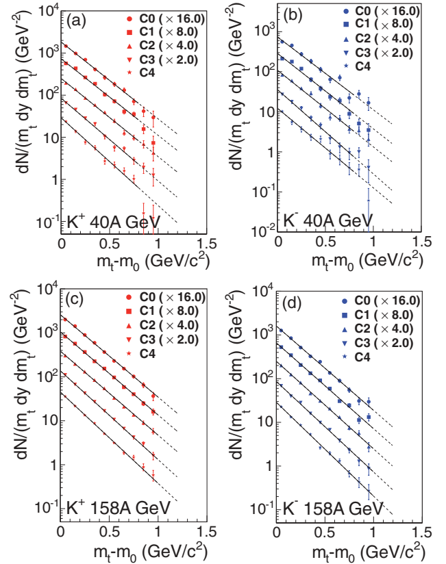
FIG. 1. (Color online) Transverse mass spectra at mid-rapidity from the combined dE/dx and TOF analysis for K^+ and K^- in Pb + Pb collisions at 40A GeV ( -0.1 < y < 0.1 ) and 158A GeV ( -0.2 < y < 0.2 ) beam energy. Lines show exponential fits for 0.0 \text{ GeV}/c^2 < m_T - m_0 < 0.8 \text{ GeV}/c^2 (40A GeV) and 0.0 \text{ GeV}/c^2 < m_T - m_0 < 1.0 \text{ GeV}/c^2 (158A GeV). Different centralities are scaled for clarity. The error bars indicate the statistical uncertainty.
