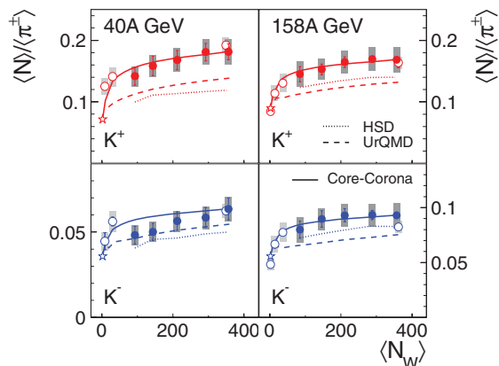
FIG. 11. (Color online) Kaon yields divided by mean number of pions \langle \pi^\pm \rangle = 0.5(\langle \pi^- \rangle + \langle \pi^+ \rangle) as a function of centrality. Closed symbols show results from centrality selected Pb + Pb collisions; open symbols show p + p data from NA49 [9,10] as well as C + C, Si + Si (at 158A GeV [8]), and central Pb + Pb collisions from [2,3]. The stars denote the values obtained from parametrization “B” in Ref. [38]. Lines show results from HSD [36] and UrQMD2.3 [37] simulations and the core-corona model (the latter for the Pb + Pb collision system only [39]). The thin vertical bars indicate the statistical errors, which are mostly not visible. The thick shaded bars indicate the systematic errors.
