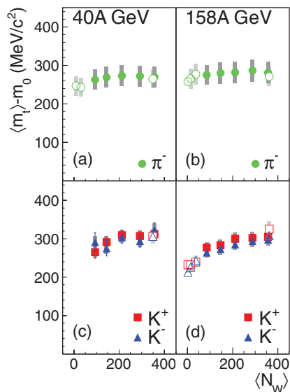
FIG. 4. (Color online) Mean transverse mass as extracted from the transverse mass spectra at mid-rapidity for \pi^- , K^+ , and K^- vs number of participating nucleons. Open symbols show results from p + p , C + C, Si + Si, and central Pb + Pb collisions. Except for the new results for C + C and Si + Si collisions at 40A GeV beam energy the data are taken from [2,3,8–10]. Filled symbols represent the centrality selected Pb + Pb data. The thin vertical bars indicate the statistical errors, which are mostly not visible. The thick shaded bars indicate the systematic errors.
