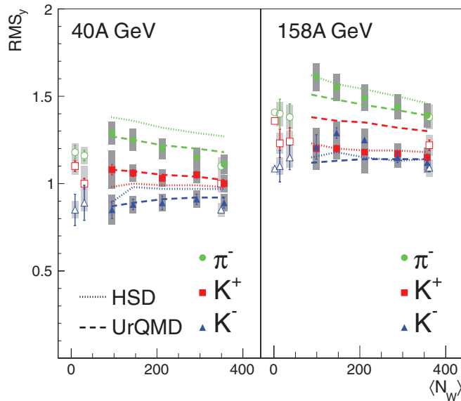
FIG. 9. (Color online) Width of the rapidity distribution described by the rms values for \pi^- , K^+ , and K^- vs mean number of participating nucleons. Open symbols show results from p + p , C + C , Si + Si , and central Pb + Pb collisions. Except for the new results for C + C and Si + Si collisions at 40A GeV beam energy the data are taken from [2,3,8,9]. Filled symbols represent the centrality selected Pb + Pb data. Lines show results from HSD [36] and UrQMD2.3 [37] simulations as indicated in the figure. The thin vertical bars indicate the statistical errors, which are mostly not visible. The thick shaded bars indicate the systematic errors.
