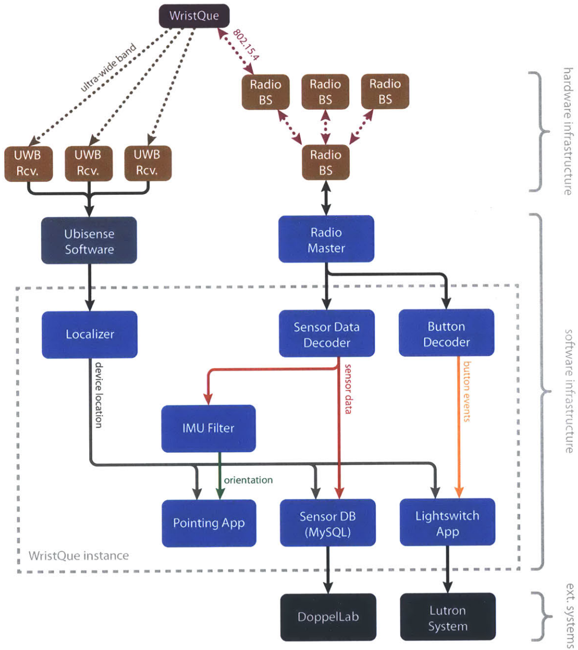
Figure 4.10: Partial system diagram of the WristQue hardware and software infrastructure.
