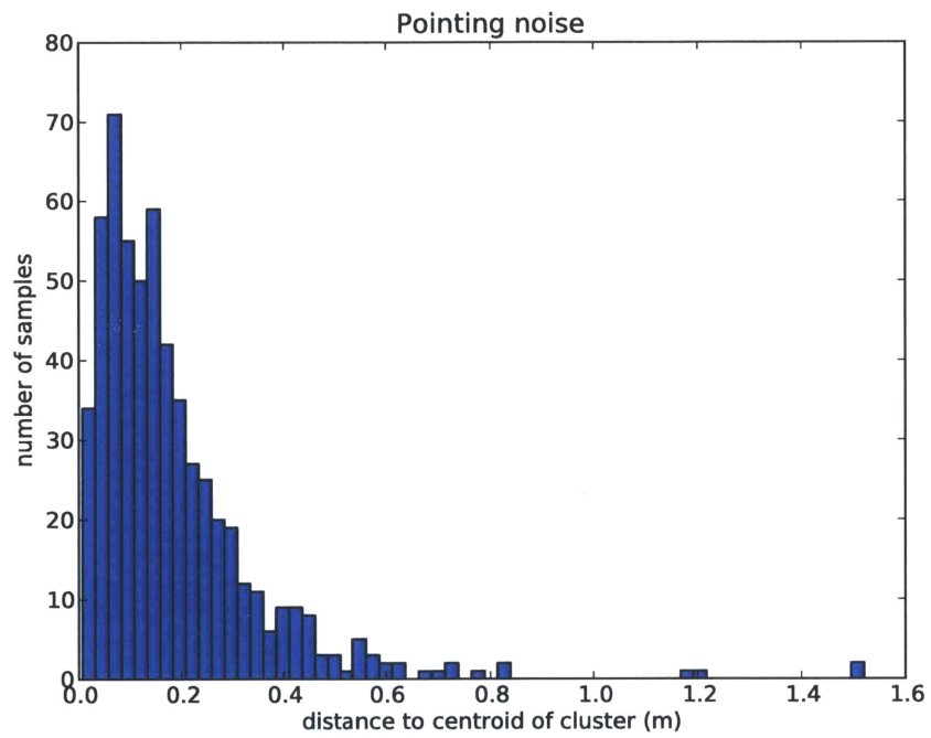
Figure 5.5: Relative noise measured in the pointing system with the user holding still and pointing at a target from different locations. The system assumes the intended target to be the centroid of the points where the ray intersects the wall plane; the histogram shows the noise between each sample and the centroid.
