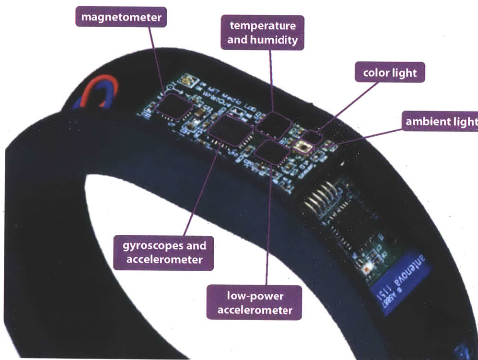
Figure 4.5: The WristQue sensor set.
