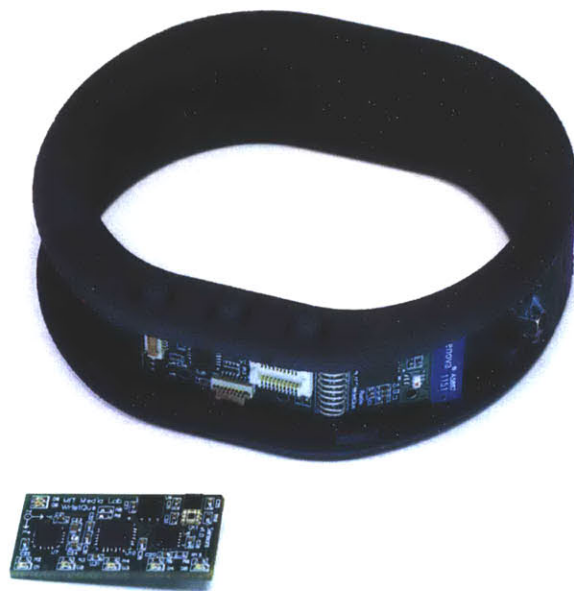
Figure 5.8: The WristQue sensor board is separate from the CPU, buttons, touch interface, and radio, allowing the sensor set to be changed without re-implementing basic functionality.
