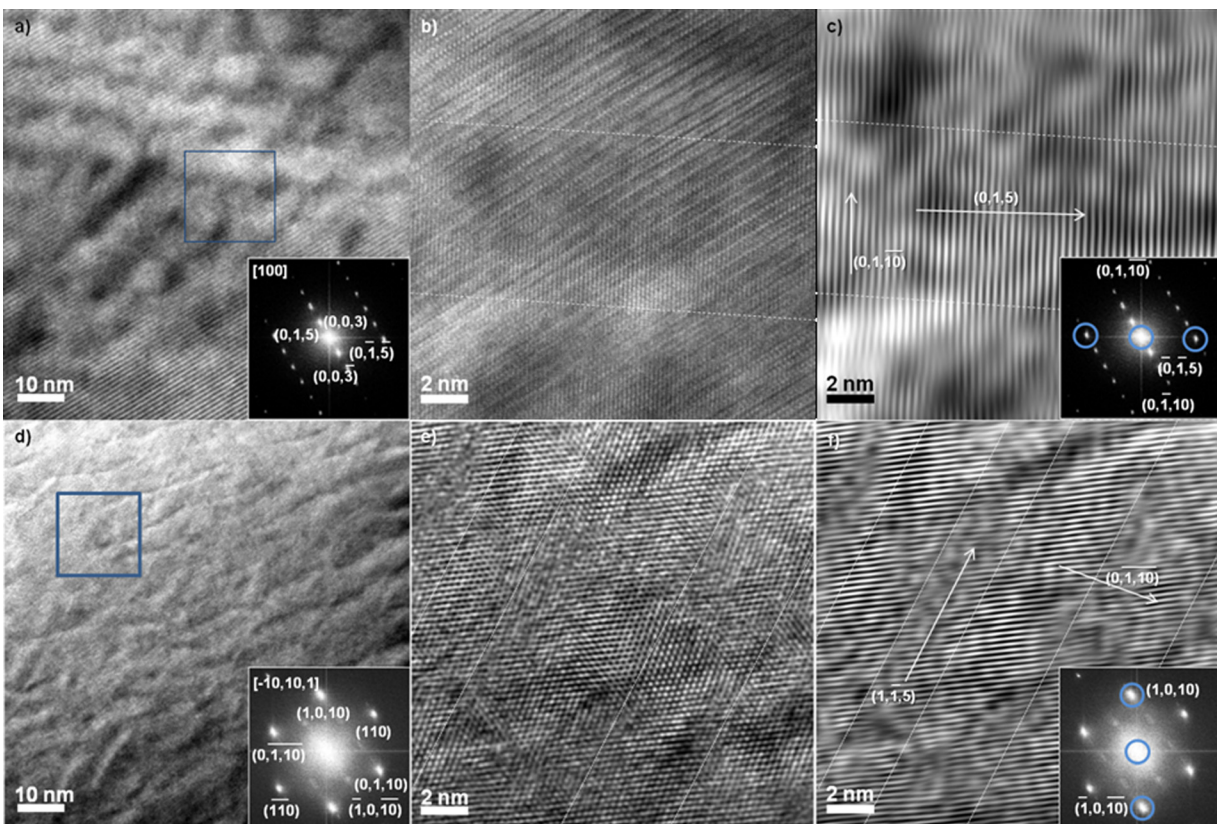
FIG. 5. (a) and (d) are zone-axis-aligned, low-magnification HRTEM images with inset FFTs of re-prepped \text{Bi}_2\text{Te}_{2.7}\text{Se}_{0.3} that was prepared via LEIT ion milling and clearly show the nanoscale structural modulation. (b) and (e) show increased magnifications of (a) and (d) respectively. (c) and (f) present FFHRTEM of (b) and (e) using g_{(0,1,5)} and g_{(1,0,10)} respectively. Alternating regions of high and low crystallinity are clearly seen in (c) and (f). Comparison of (c) and (f) with (a) and (d) demonstrates that the alternating light/dark contrast of the low magnification images is associated with the alternating high and low crystallinity of the Fourier filtered images.
