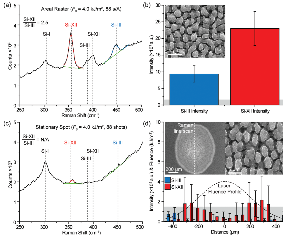
FIG. 2. (a) A representative Raman spectrum from a rastered surface that received 88 s/a with a peak fluence, F_0 , of 4 kJ/m 2 . The background (green) and fits to the Si-XII mode (red) and the Si-III mode (blue) are overlaid. (b) The average intensity and standard deviation of the Si-III (blue) and Si-XII (red) Raman modes from 20 spectra collected from the rastered surface; SEM image of the surface morphology is shown in inset. (c) A representative Raman spectrum from a stationary laser-irradiated spot that received 88 pulses with a peak fluence of 4 kJ/m 2 , with background (green) and a fit to the Si-XII mode (red) overlaid. The Si-III mode is not detectable. The spectrum corresponds to the position 300 μm from the center of the laser spot. (d) The average intensity and standard deviation of the Si-III and Si-XII Raman mode intensity measured across the stationary laser-irradiated spot (left inset) along with the varying laser fluence. The surface morphology at the center of the laser-irradiated spot is shown in the right inset. Line scans were obtained across 5 different laser spots and then spatially binned to illustrate trends. In both (b) and (d), the error bars represent one standard deviation and the gray regions indicate the peak fitting noise floor (1500 a.u.).
