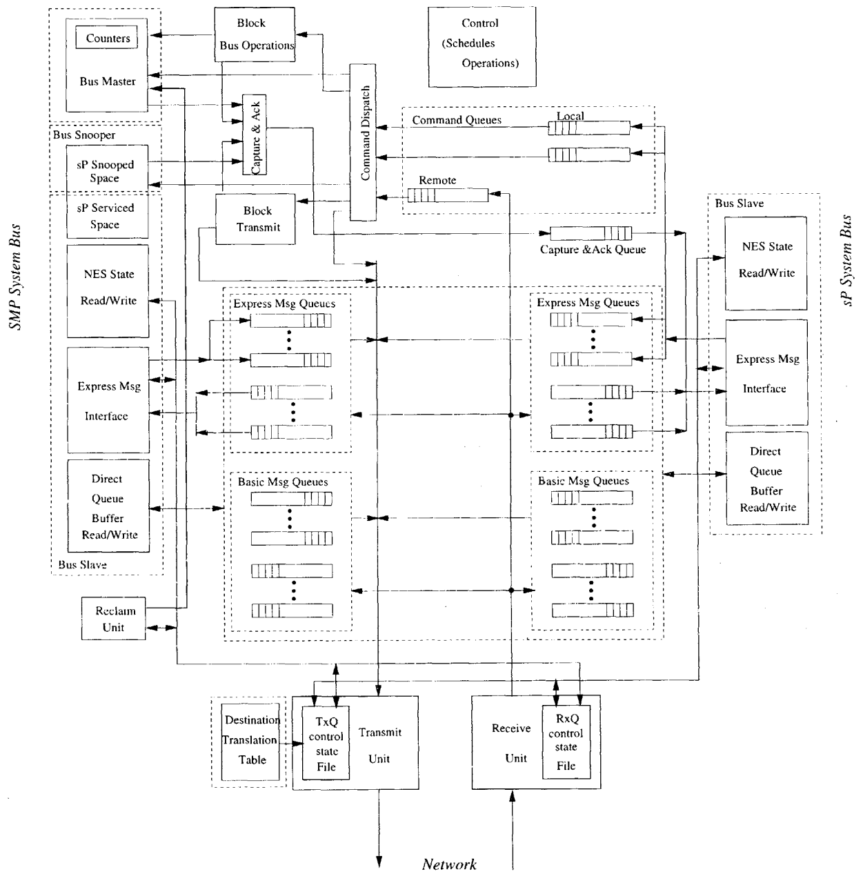
Figure 4-8: Queues and functional units in the StarT-Voyager NES.
