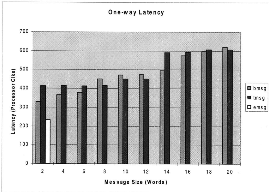
Figure 5-1: One-way latency for Express (emsg), Express-TagOn (tmsg) and Basic (bmsg) messages as message size varies from 2 to 20 (4 byte) words.
