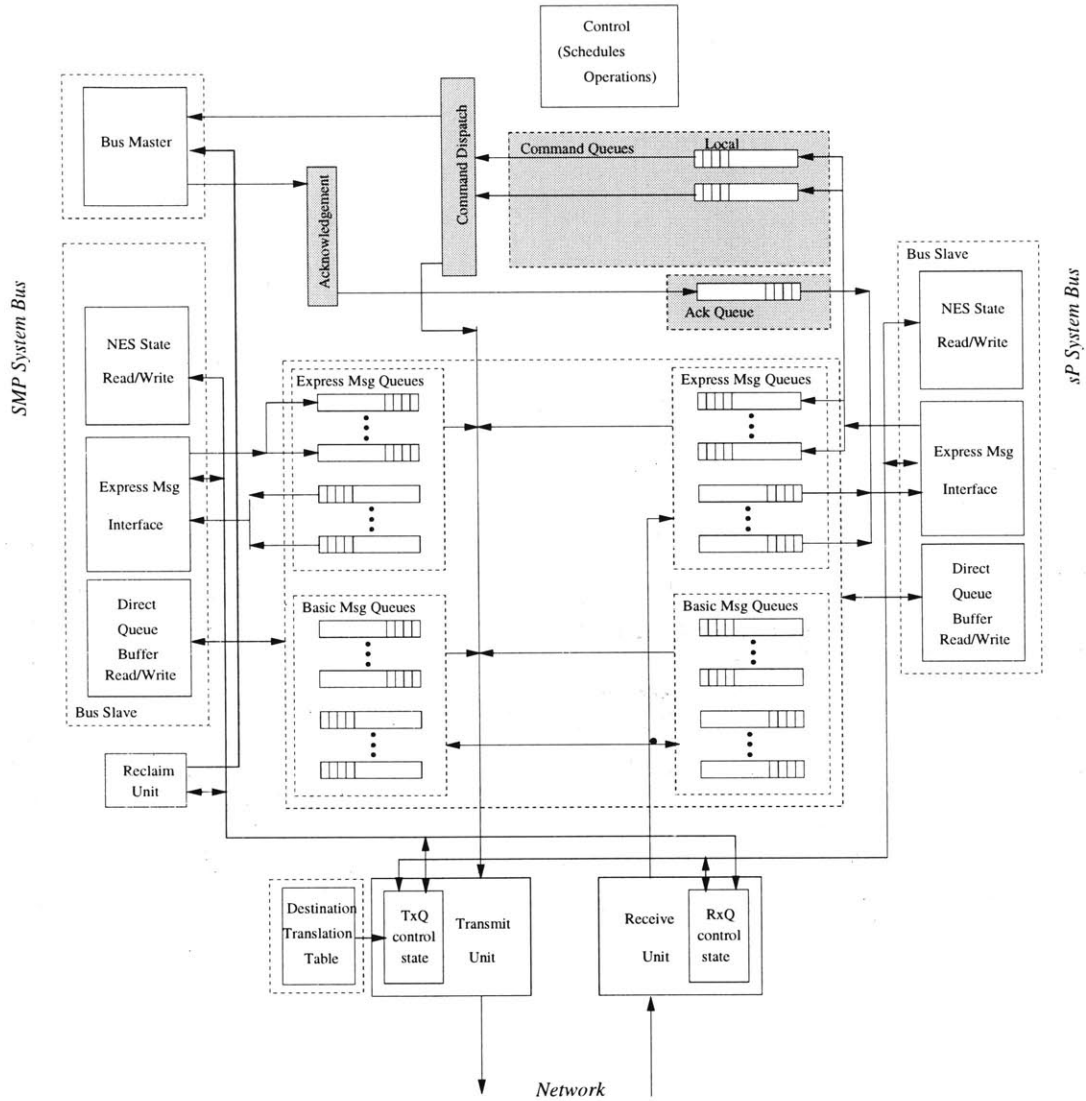
Figure 4-18: Queues and functional units to implement Resident Express message, Basic message (including Reclaim), and giving sP the ability to initiate bus transactions on the SMP system bus. The latter is made possible with the addition of the shaded regions.
