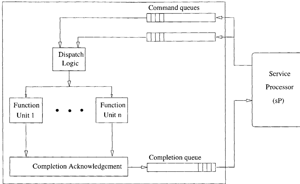
Figure 4-6: A command and completion queues interface.
