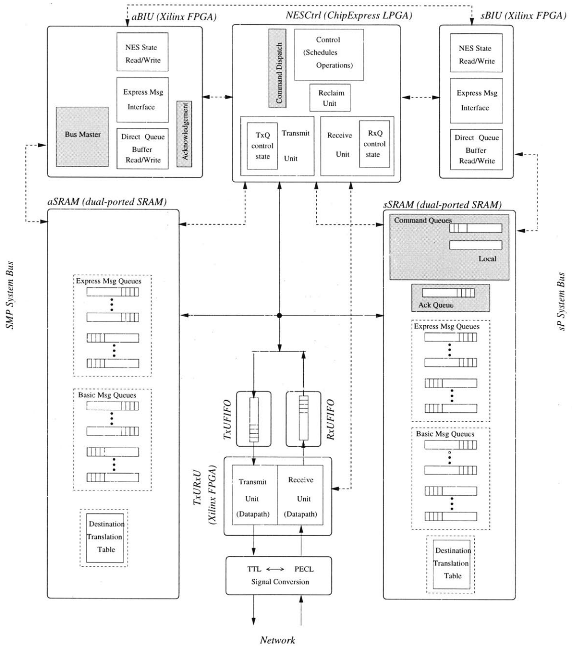
Figure 4-19: Actual realization of Resident Express and Basic message functions (including Reclaim), and giving sP the ability to initiate bus transactions on the SMP system bus. The latter is made possible with the addition of the shaded regions.
