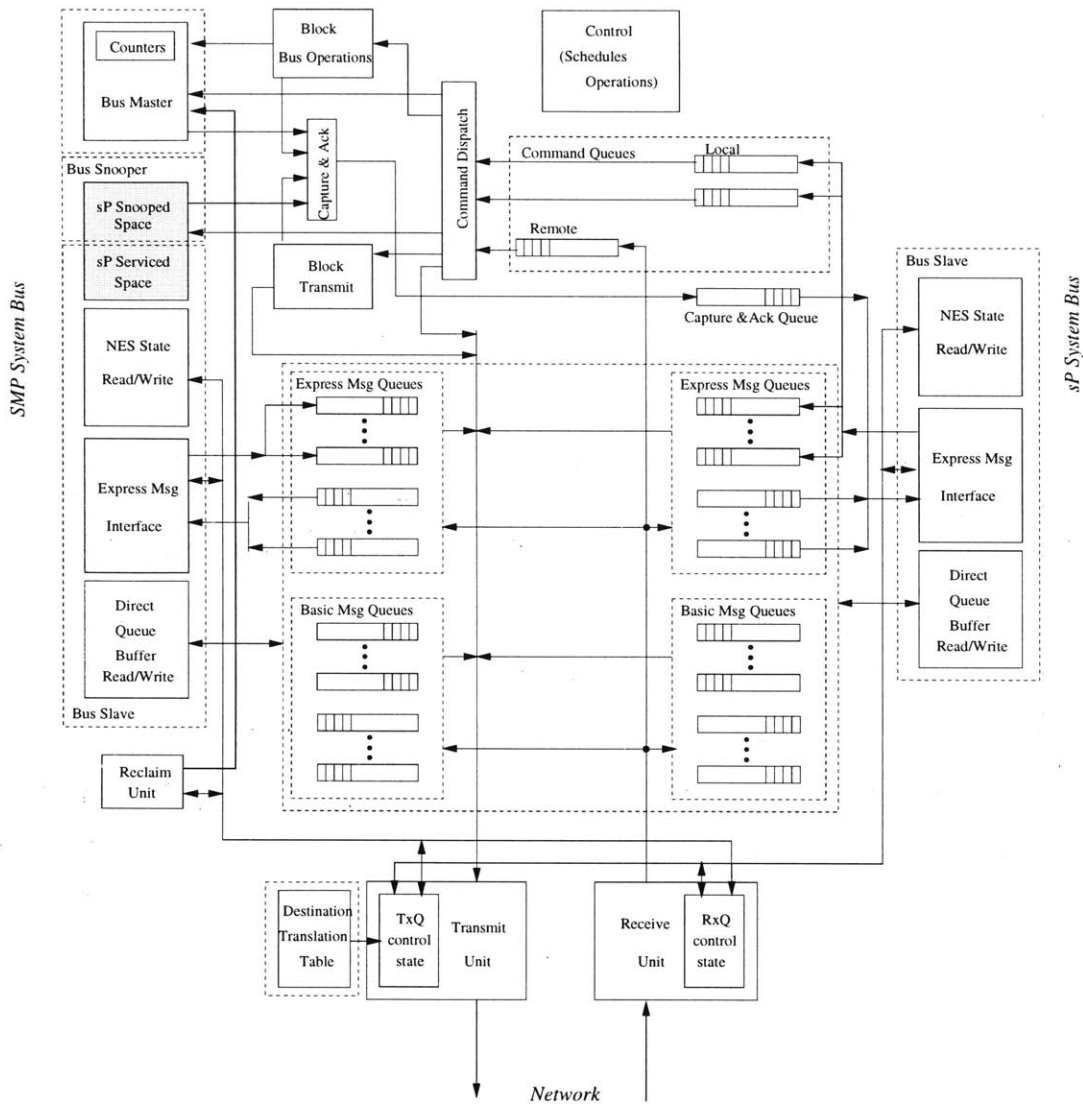
Figure 4-25: This diagram illustrates the addition of Snooped Space support through the shaded functional block. It also shows the full design of the StarT-Voyager NES.
