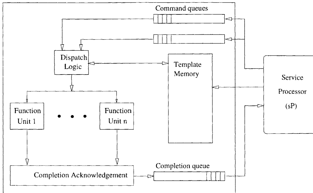
Figure 4-7: A template augmented command and status register interface.
