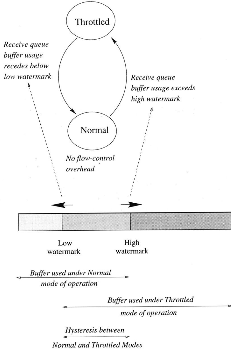
Figure 3-4: Overview of Reactive Flow-control.
