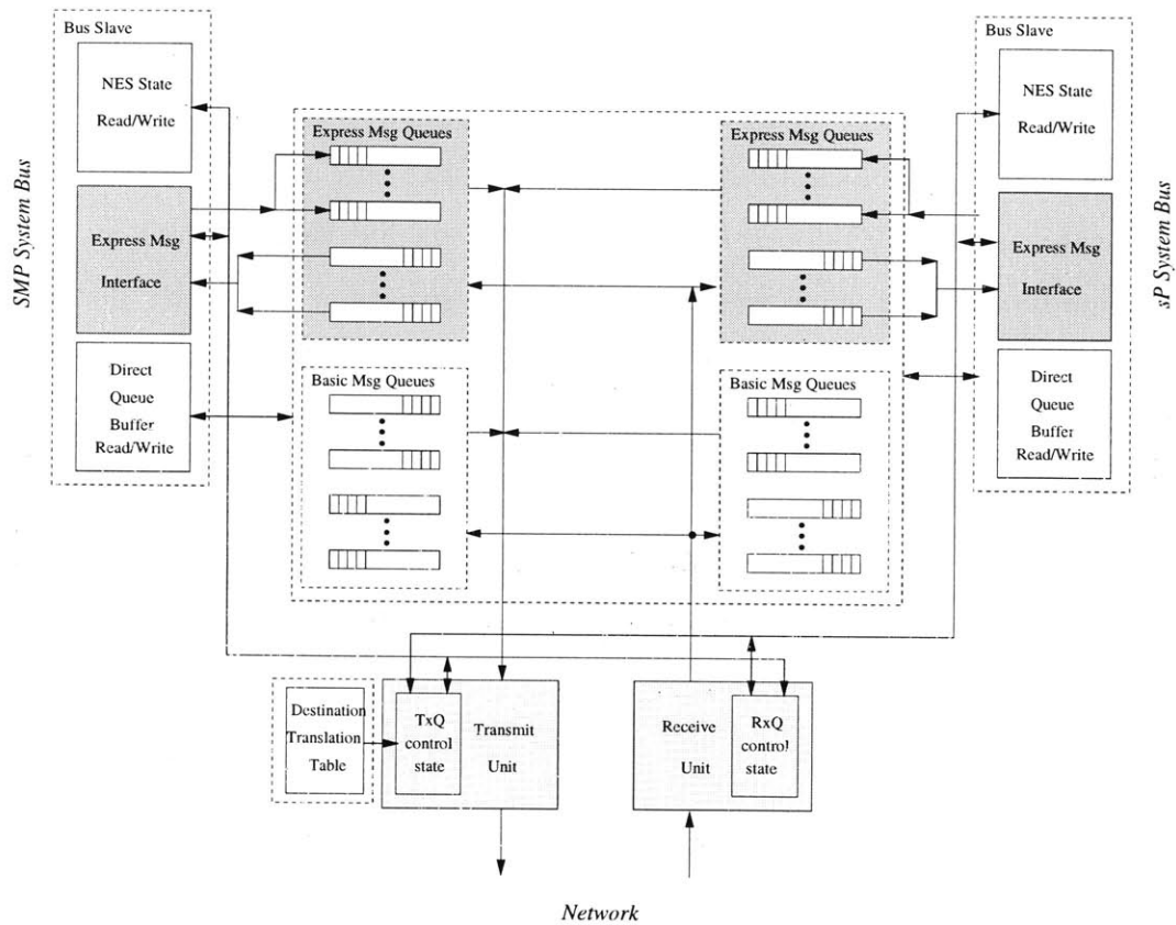
Figure 4-12: Queues and functional units to implement Resident Express message and Basic message. The lightly shaded portions require modifications when we add Express message. The more deeply shaded portions are new additions for Express message.
