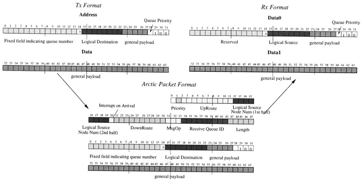
Figure 3-6: Express Message Formats
