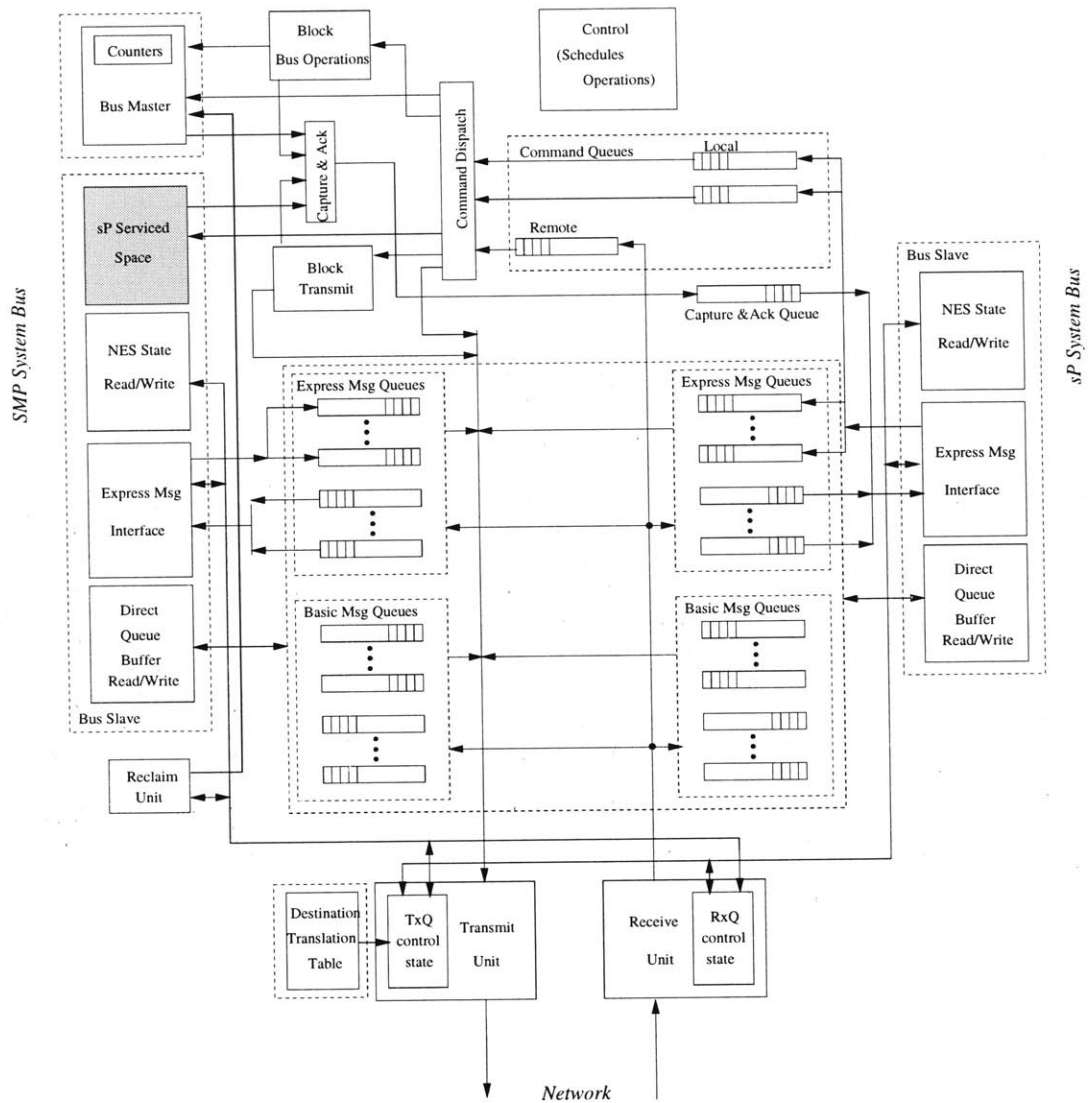
Figure 4-22: The addition of sP Serviced space support to the NES involves introducing the shaded functional block. Other existing infrastructure, such as the Capture & Ack queue, is re-used.
