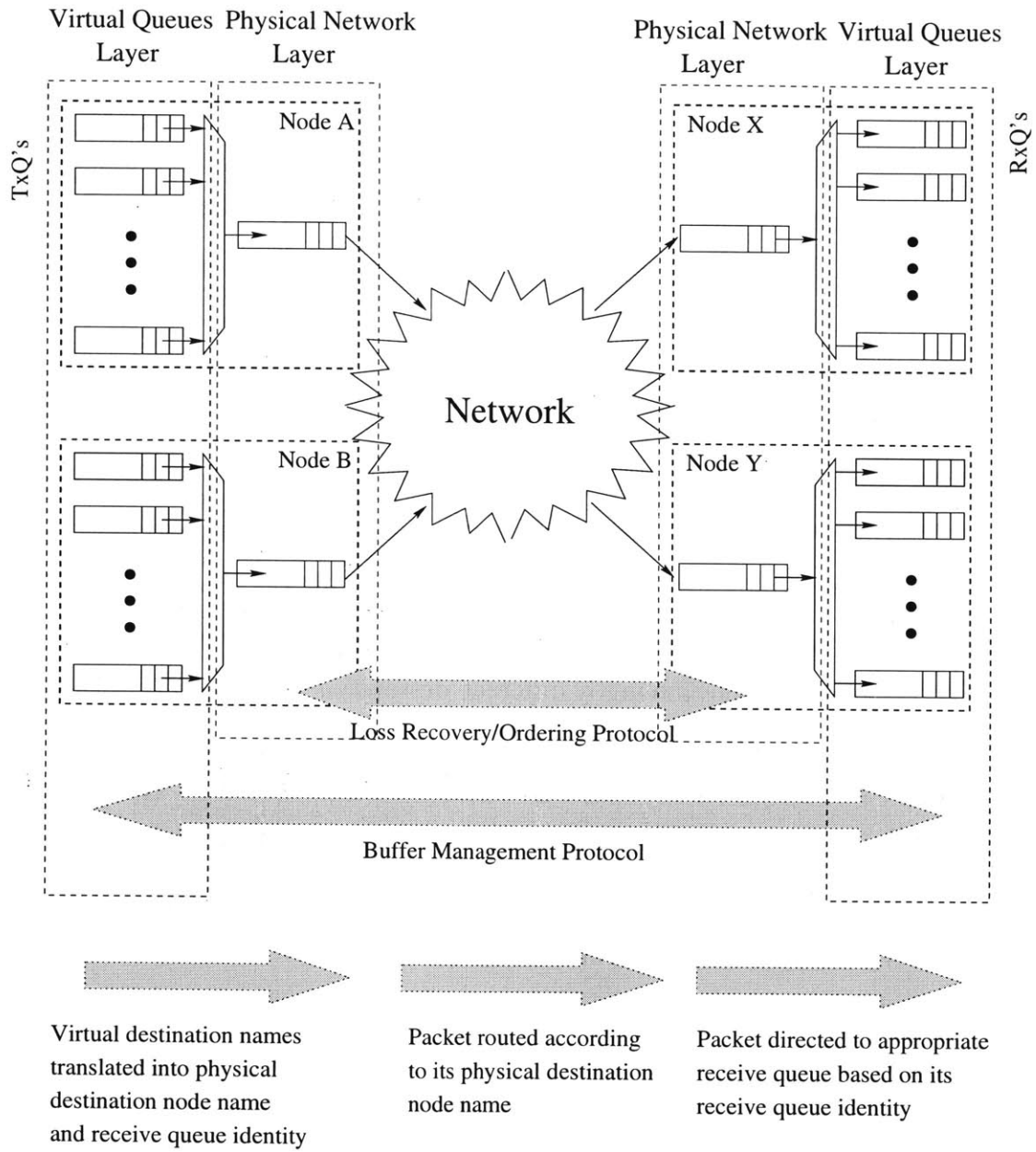
Figure 3-2: Relationship between the Virtual Queues layer and Physical Network layer.
