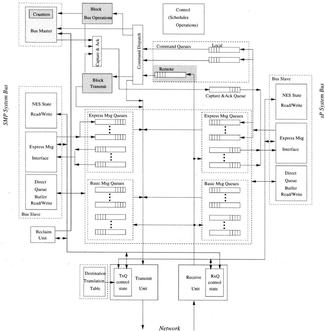
Figure 4-20: This diagram illustrates the addition of DMA support. The lightly shaded blocks are modified while the darkly shaded regions are new additions to provide NES hardware DMA support.
