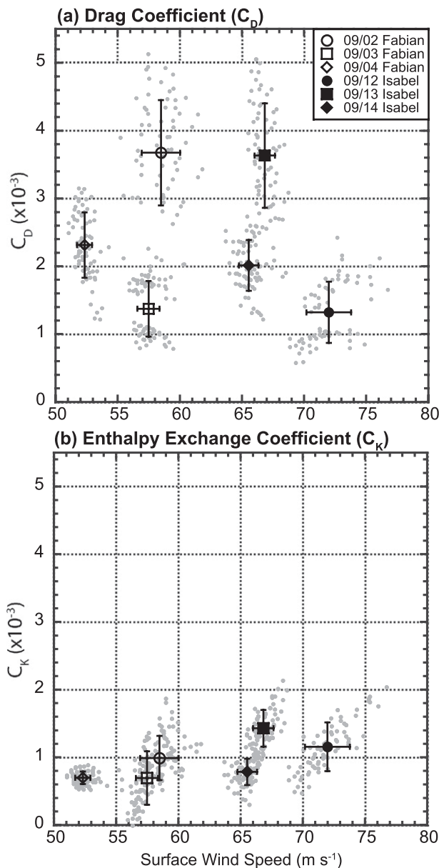
FIG. 16. Derived 10-m bulk exchange coefficients from the absolute angular momentum and total energy budget retrievals. Symbols are as in Fig. 14.
