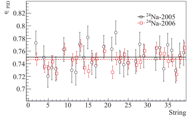
FIG. 6. (Color online) \epsilon_{PID} as a function of string for the ^{24}\text{Na} calibration data. Fits to straight lines give 0.7505 \pm 0.0035 with \chi^2/\text{NDF} of 24.1/29 and 0.7467 \pm 0.0018 with \chi^2/\text{NDF} of 49.3/29, respectively.
