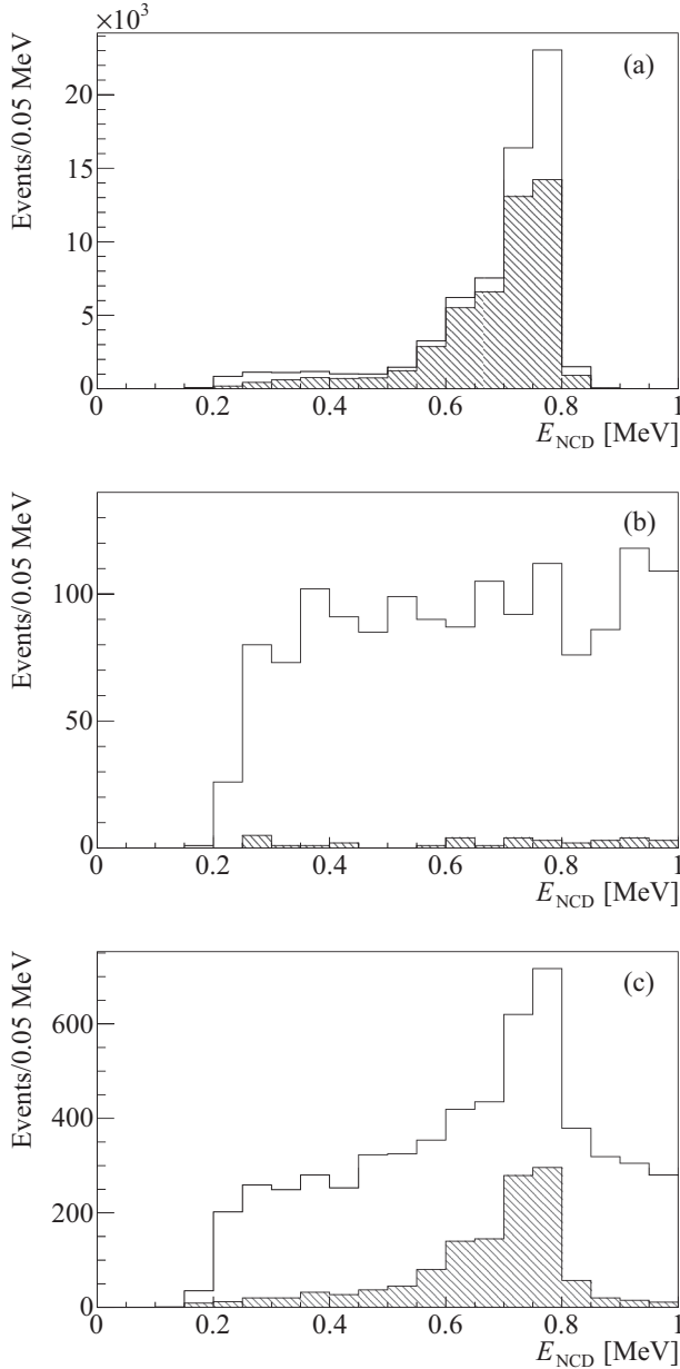
FIG. 5. E_{NCD} spectrum before (white) and after (hashed) the particle identification cut. (a) is for ^{24}\text{Na} calibration data (neutrons). (b) is for data from strings filled with ^4\text{He} (alphas). (c) is for data from strings filled with ^3\text{He} .
