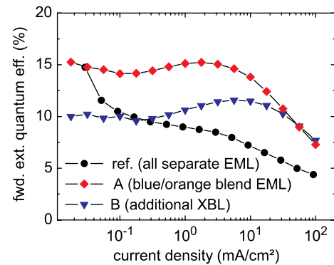
FIG. 25 (color online). External quantum efficiency vs current density for different triplet-harvesting integrations (bilayer and blended systems) showing strong differences in the efficiency roll-off. XBL is the exciton blocking layer. From Schwartz, Reineke et al. , 2008.
