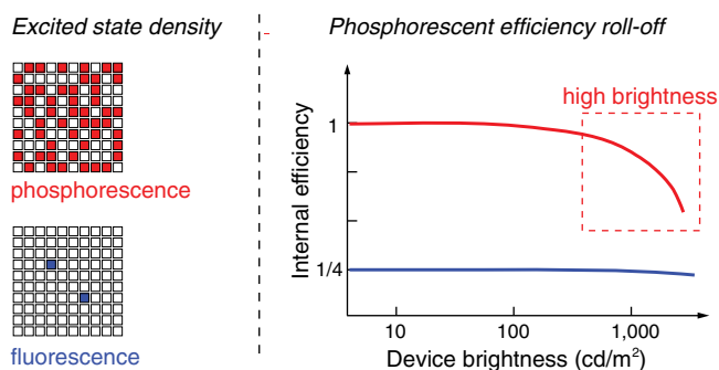
FIG. 5 (color online). Left: The excited-state density in the cases of phosphorescence and fluorescence, respectively. Right: Typical efficiency vs. brightness characteristics. In the case of phosphorescence, the efficiency drastically decreases at high brightness as a consequence of quenching processes.
