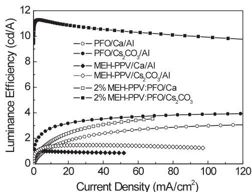
FIG. 15. Current efficiency of three sets of devices. The composition of the EML and the interfacial electron injection layer are varied. (To our knowledge, the labels of the last two devices are incomplete. They should both contain an “/Al” cathode.) From Huang, Li et al. , 2006.
