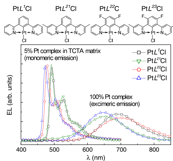
FIG. 36 (color online). Top: Molecular structures of different emitters. Corresponding EL spectra of all emitters obtained for a 5 wt % host-guest system (TCTA host) and a pure film EML formed by the platinum complexes. Each spectrum is normalized to the integrated intensity. From Cocchi et al. , 2009.
