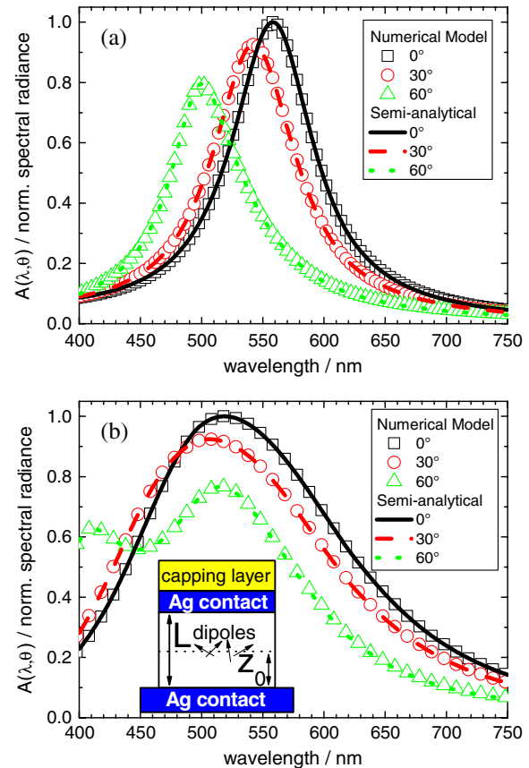
FIG. 47 (color online). Calculated extractable power A(\lambda, \theta) of two model OLED structures having the following layer sequence: (a) 100 nm Ag/100 nm organic ( n = 1.8 )/15 nm Ag. (b) Layer structure of (a) followed by an additional 50 nm organic capping layer. Emitters are placed in the field antinode corresponding to a resonance wavelength of approximately 560 nm. From Thomschke et al. , 2009.
