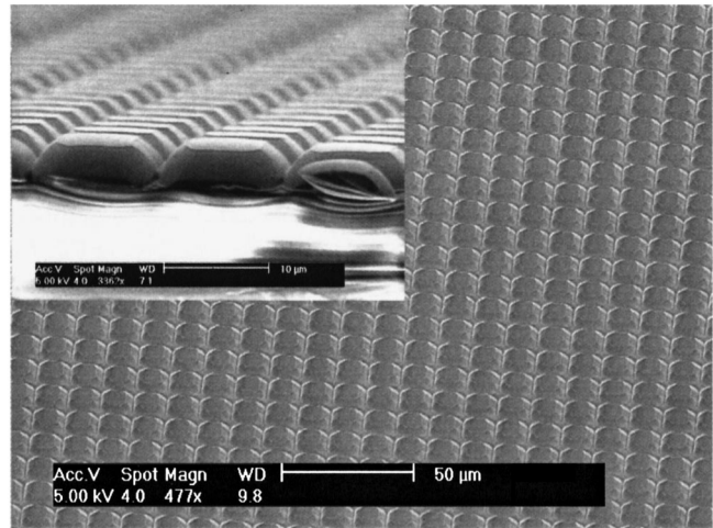
FIG. 39. Scanning electron micrograph of a PDMS microlens array using an etched \text{SiN}_x mold. Inset: Side view. The base lengths of the lenses are approximately 10\ \mu\text{m} . From Möller and Forrest, 2002.
