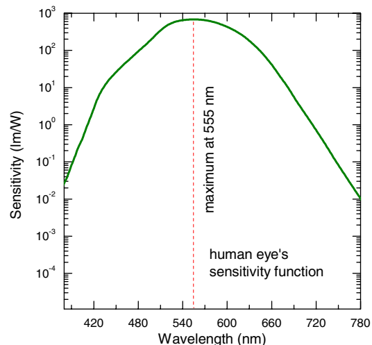
FIG. 6 (color online). Commission Internationale de l'Éclairage (CIE) photopic (daylight) spectral sensitivity function V(\lambda) . Its maximum at a wavelength of 555 nm corresponds to 683 \text{ lm W}^{-1} .
