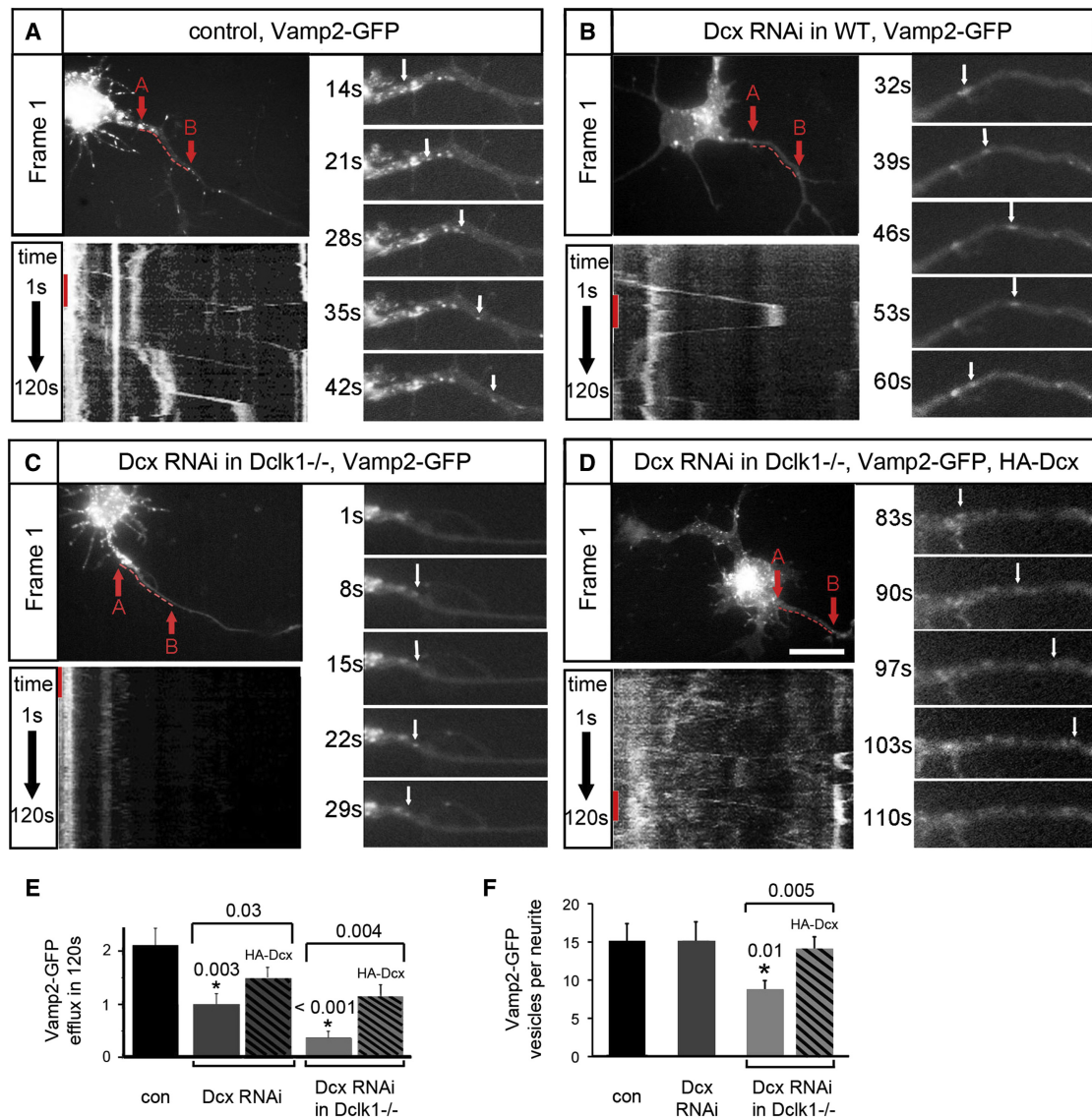
Figure 3. Efflux of Vamp2-GFP into Neurites Is Impaired in Dcx/Dclk1-Deficient Neurons
