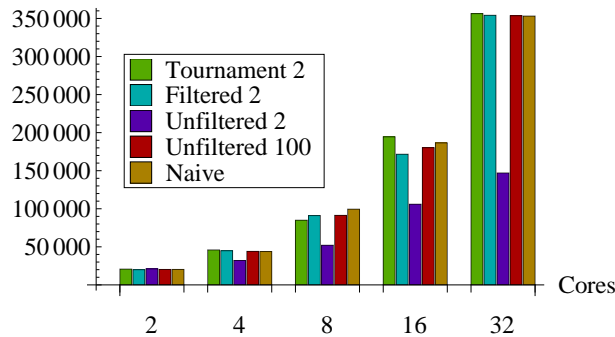
Figure 8: Scaling of connections per second with different load balancing schemes under a uniform workload. Naïve performs no load balancing – connections are always sent to the local web server. All load balancing schemes except Unfiltered 2 match naïve scaling.
