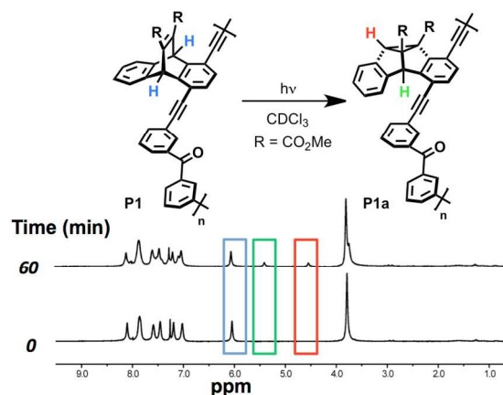
Figure 5. Di- \pi -methane rearrangement of P1 (top). Time-elapsing ^1\text{H} NMR spectra of the reaction (bottom).
