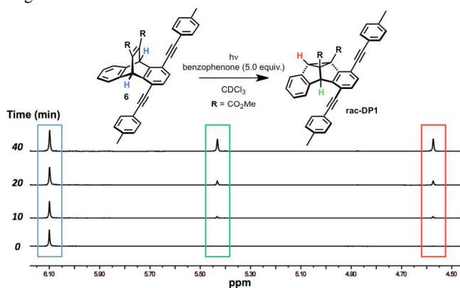
Figure 4. Di- \pi -methane rearrangement of model compound 6 (top). Time-elapsing ^1\text{H} NMR spectra recorded during the sensitized photolysis of 6 (bottom). The intensity is normalized to the resonance at 6.1 ppm.
