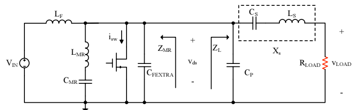
Fig. 10. Class \Phi 2 inverter. L_S is a resonant inductor.
