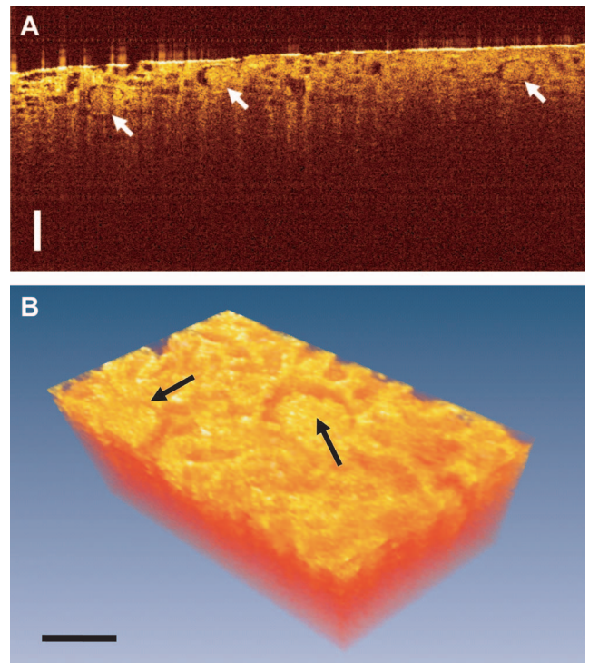
Fig. 8 (a) Cross-sectional OCT image revealing several glomeruli (arrows) subjacent to the surface of the kidney. Bar: 250 \mu\text{m} . (b) Three-dimensional reconstruction of OCT images seen in (a) reveals two glomeruli (arrows) and the surrounding capsular spaces of Bowman. Size: 1.7 mm (L) \times 0.9 mm (W) \times 1.0 mm (D). Bar: 100 \mu\text{m} .
