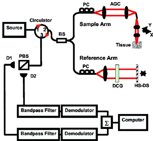
Fig. 1 Schematic of the high-resolution OCT system. BS: 90/10 fiber-based beamsplitter; PC: polarization controller; AGC: air-gap coupling; DCG: dispersion compensating glass; HS-DS: high-speed delay scanner; PBS: polarization beamsplitter; D: detector; \Sigma : vector summation.
