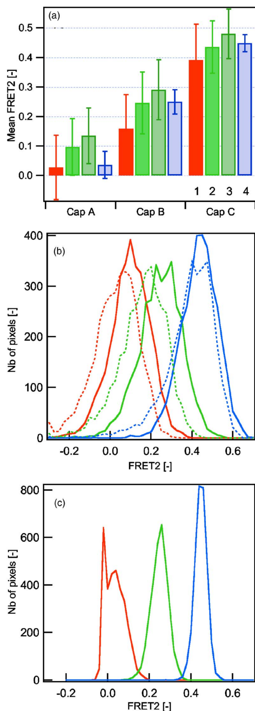
Fig. 4 (a) Mean FRET 2 indices retrieved in each capillary with different data analysis techniques. 1. Two-channel algorithm, 2. spectral imaging with spectral decomposition, 3. spectral imaging split for two channel algorithm, and 4. global fitting of FLIM data. (b) FRET 2 histogram for spectral imaging with decomposition (solid lines) and two-channel (dotted line) imaging in capillaries A, B, and C (in ascending order). (c) FRET 2 histogram for FLIM in capillaries A, B, and C.
