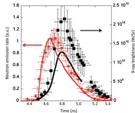
FIG. 3 (color online). Measured (symbols) and calculated (lines) x-ray (black) and neutron (red) emission from the low convergence implosion.
