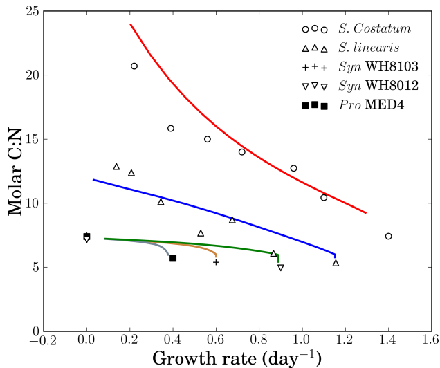
Figure 6. Model–data comparison of whole cell C:N ratio under conditions of nutrient-limited, balanced growth. In all cases, the C:N ratio increases as nutrient supply diminishes. S. costatum (Sakshaug et al., 1989) have a higher C:N ratio by comparison to S. linearis (Healey, 1985) and other cyanobacteria (Bertilsson et al., 2003) at very low growth rates. The red, blue and green lines are model predictions for cell sizes corresponding to S. costatum , S. linearis and WH8012, respectively. Gray and brown lines are model predictions of Prochlorococcus MED4 and Synechococcus WH8103. Modeled PFD matched the experimental conditions, which were 30–40 \mu\text{mol photons m}^{-2} \text{s}^{-1} for MED4, WH8012, WH8103; 80 \mu\text{mol photons m}^{-2} \text{s}^{-1} for S. linearis and S. costatum . S. linearis and S. costatum were N limited in chemostats, whereas MED4, WH8012 and WH8103 were P limited in batch culture. These data may be less than the nitrogen-limited C:N if, for example, P-limited organisms are still able to accumulate inorganic N.
