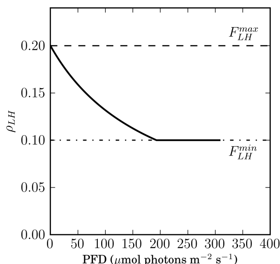
Figure 4. Demonstration of the modeled regulation of nitrogen allocation to light harvesting with Eq. (9). There is a non-linear reduction in light-harvesting apparatus as a function of PFD (see also Fig. 5). Parameters for this figure: F_{LH}^{min} = 0.1 , F_{LH}^{max} = 0.2 and F_{LH}^G = 0.06 .
