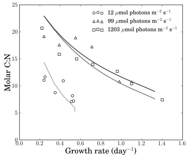
Figure 7. Dependence of C:N on nitrogen-limited growth rate for the diatom S. costatum under a range of light intensities (Sakshaug et al., 1989). Symbols are experimental measurements, and gray lines are model results. The modeled light conditions matched the experimental conditions. Even when grown under extremely low PFD, S. costatum has a much wider range in C:N than the oceanic cyanobacteria in Fig. 6.
