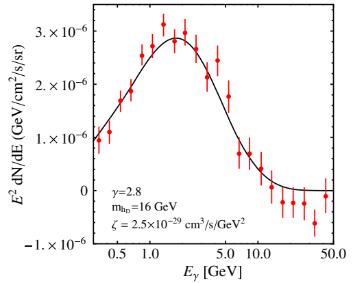
FIG. 4 (color online). DM parameters which allow an interpretation of the Galactic center gamma ray excess. The red data points show the excess extracted in Ref. [90] and the black line is the spectrum from boosted h_D decays. The possible realization of these parameters in specific models is discussed in the text.
