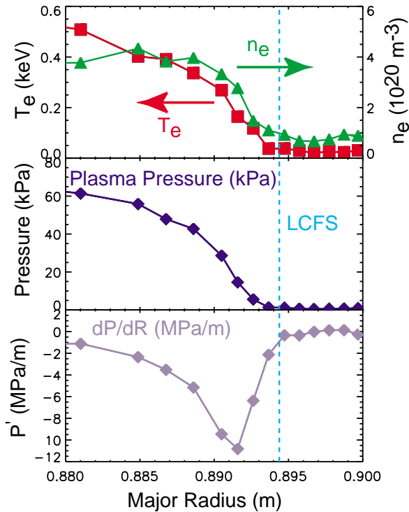
FIG. 7. T_e and n_e profiles from high resolution edge Thomson scattering. The pressure profile is constructed assuming T_i = T_e .
