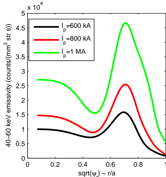
FIG. 6. (Color online) Inverted HXR spectra from discharges with 3 different plasma currents: 600 kA, 800 kA, and 1 MA. Plasma parameters for this experiment were B=5.4 \text{ T} , \bar{n}_e = 9 \times 10^{19} \text{ m}^{-3} . T_{e0} for the 600 kA, 800 kA, and 1 MA discharges was 1.9, 2.3, and 2.1 keV respectively. As the current increased from 600 kA to 1 MA, The loop voltage increased from 0.8 to 1.1 V. The launched n_{||}=3.1 for these discharges.
