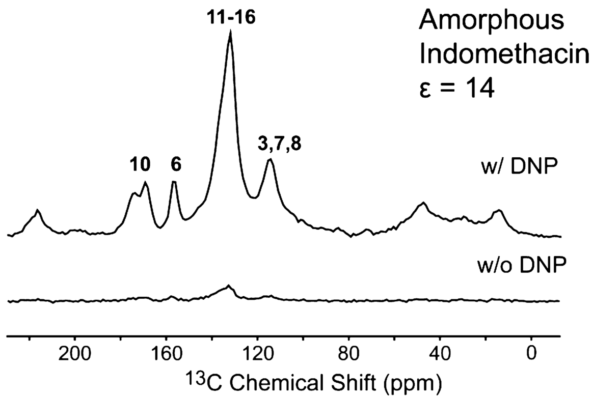
Figure 7. ^{13}\text{C} CPMAS DNP enhanced spectra of indomethacin glass doped with 0.5 mol % bTereph.
