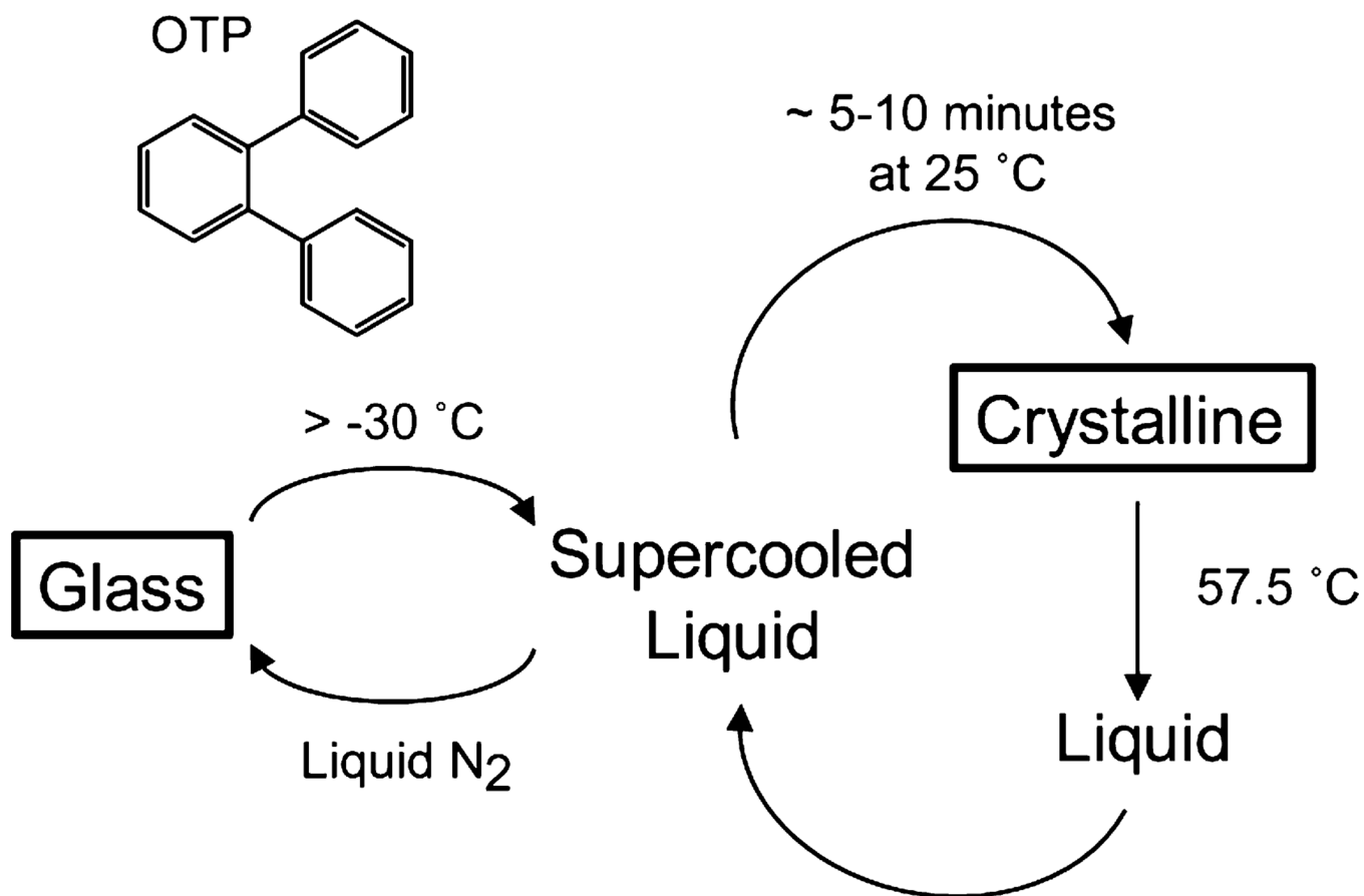
Figure 1. Phase transition scheme of ortho -terphenyl (OTP).
