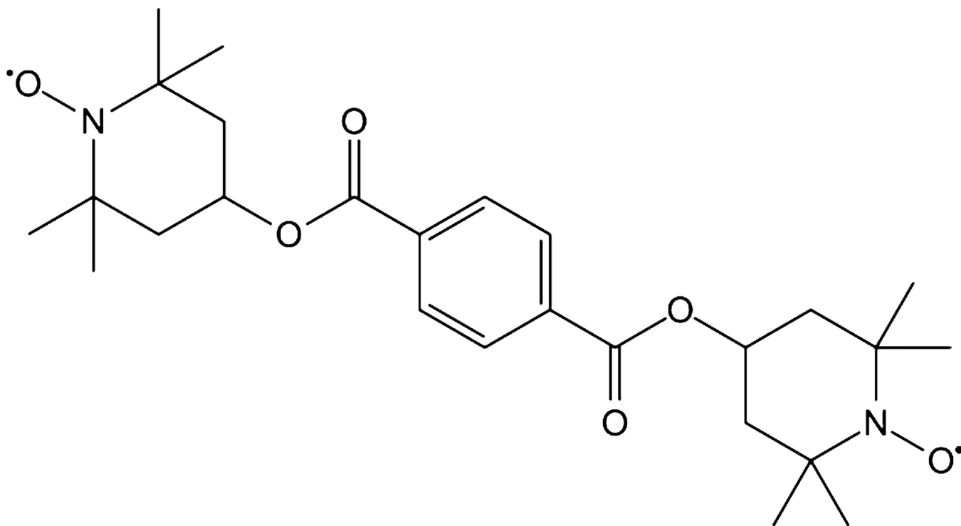
Figure 3. Structure of bis-TEMPO terephthalate (bTtereph).
