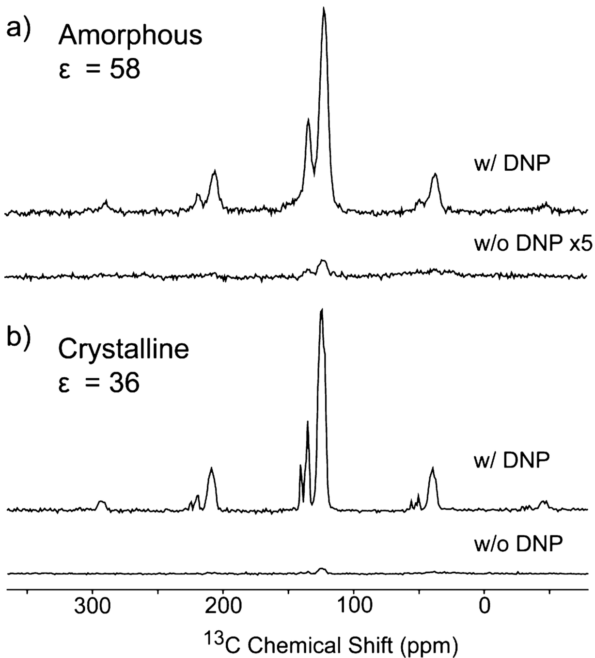
Figure 4. ^{13}\text{C} CPMAS DNP enhanced spectra of 95% deuterated OTP with 0.5 mol % bTereph for the (a) amorphous and (b) crystalline states. The spectra are plotted with the DNP off spectra (no microwaves) to demonstrate the increase in signal-to-noise.
