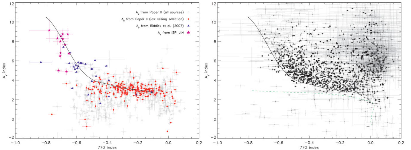
Figure 11. Color–color plot expressed in units of [770 index] (reddening independent) and [ A_V index] (parallel to the reddening direction). Left panel: sample of extinction-corrected sources; A_V values are from Riddick et al. (2007), the JHK photometry of Robberto et al. (2010), and the optical analysis of Paper II. For the latter, accretors and candidate non-accretors are distinguished as in Figure 8. The solid line represents our best fit of the data, i.e., the empirical isochrone for A_V = 0 . Right panel: same diagram, reporting all the sources in our catalog, with no correction for extinction. These are color coded according to their photometric errors. The entire population, with the exception of very few sparse sources, is located above the isochrone, at positive values of extinction.
