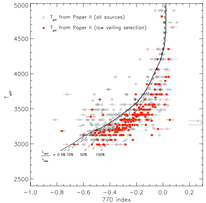
Figure 9. Same as Figure 8, showing the displacement in the reddening-independent [770 index] obtained by adding an amount of accretion luminosity to the star. The thick line is the isochrone from Paper II, the same model shown also in Figure 5. The dashed lines are the same model, after the addition of a given amount of accretion luminosity to each synthetic spectrum, for different values of \log L_{\text{accr}}/L_{\text{tot}} . Note that the fact that the red dots are low accretion sources, whereas the model requires a large value of L_{\text{accr}} to predict their colors, implies that the base isochrone needs adjustments (see the text).
