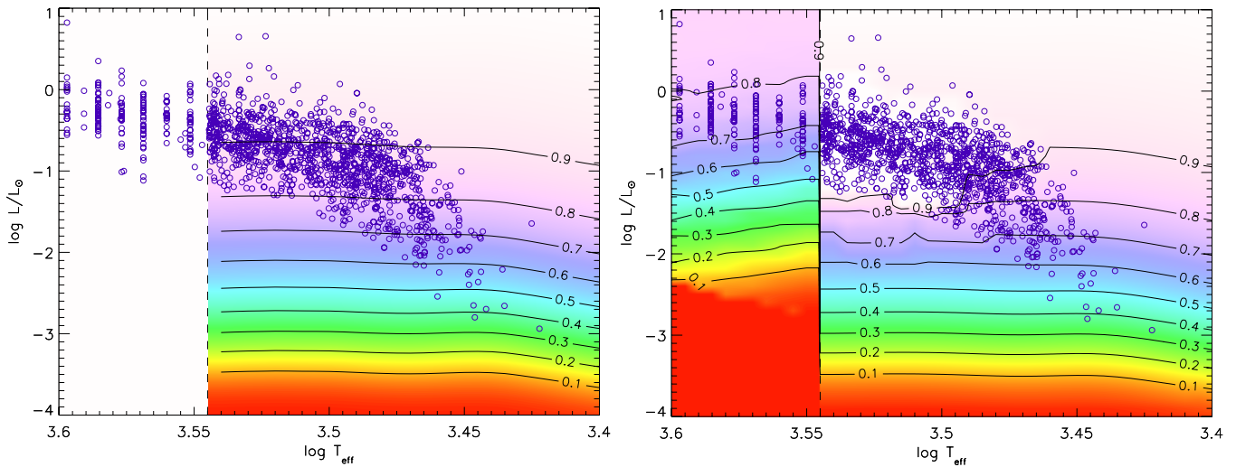
Figure 17. Completeness function in the H-R diagram, computed accounting for photometric detection and differential reddening as described in the text. The left panel shows the result as computed with our Monte Carlo simulation, valid for the spectral types obtained from the medium-band photometry analyzed in this work, for \log T_{\text{eff}} < 3.54 ( T_{\text{eff}} < 3500 K). The right panel shows the correction of this completeness after accounting for the additional stars placed in the HRD whose stellar parameters are taken from Paper II. (A color version of this figure is available in the online journal.)
