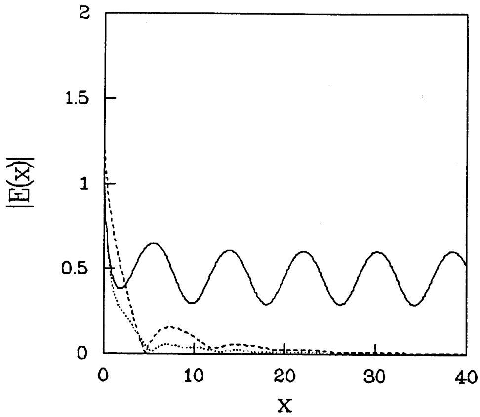
FIG. 4. Periodic state: Spatial profile of the amplitudes at a fixed time at (1,1).
