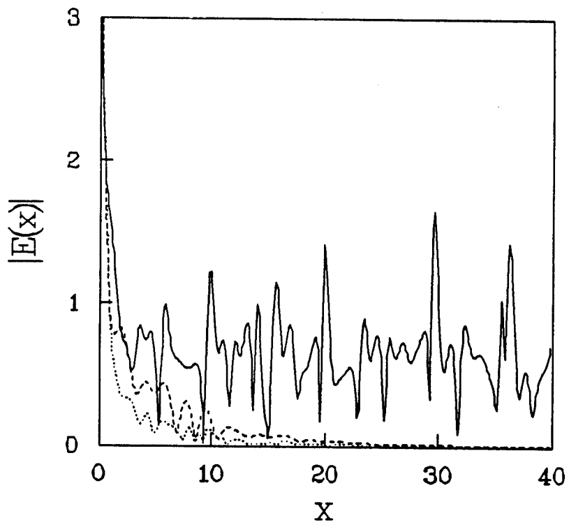
FIG. 12. Chaotic state: Spatial profile at (1,5).
