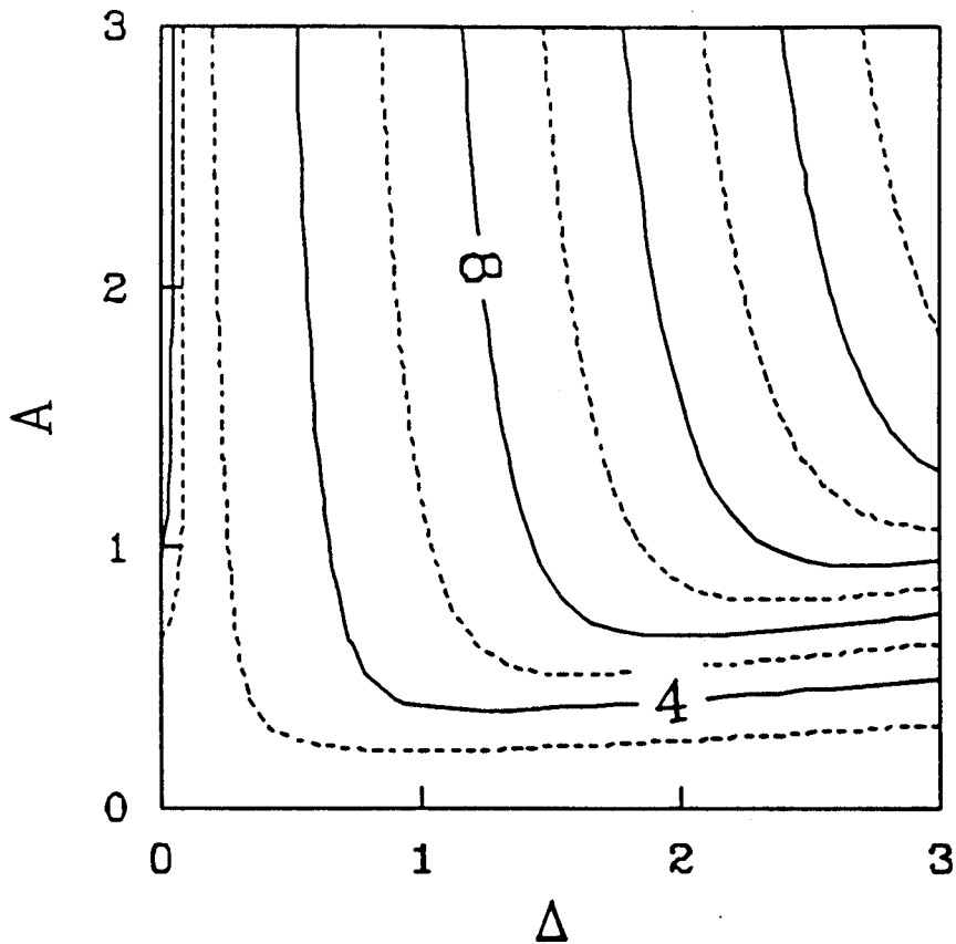
FIG. 3. Contour plot of \phi_s(x = 0) in the \Delta - A plane for L = 40 , \epsilon = 0.0025 .
