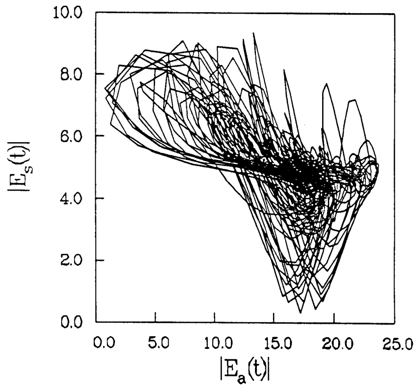
FIG. 10. Chaotic state: Phase Portrait at (1,5).
