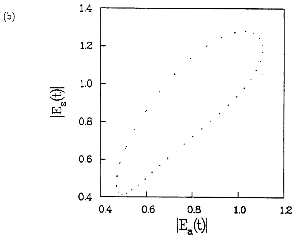
FIG. 6. Periodic state: (a) Phase portrait E_s vs. E_a at (1,1); (b) Phase portrait strobed at t_n = 2\pi/\Delta .
