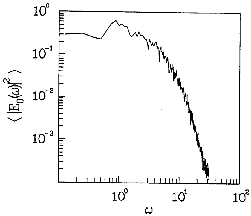
FIG. 11. Chaotic state: Power spectrum of the pump at (1,5).
