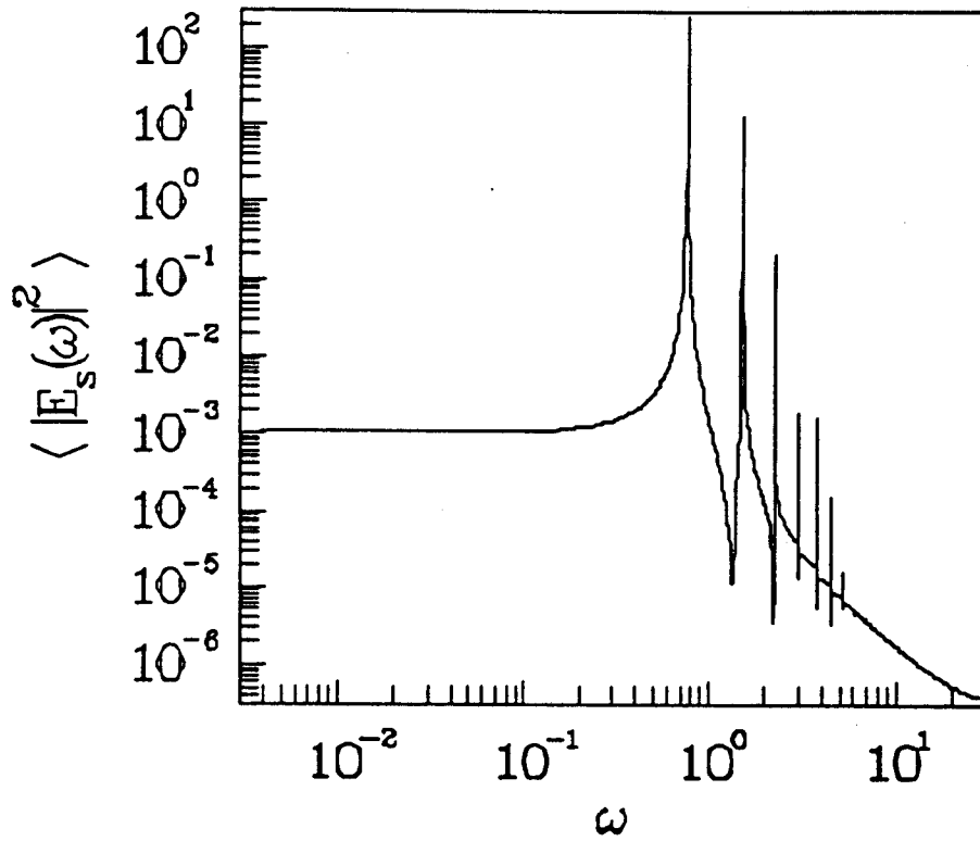
FIG. 5. Periodic state: Power spectrum of pump at (1,1).
