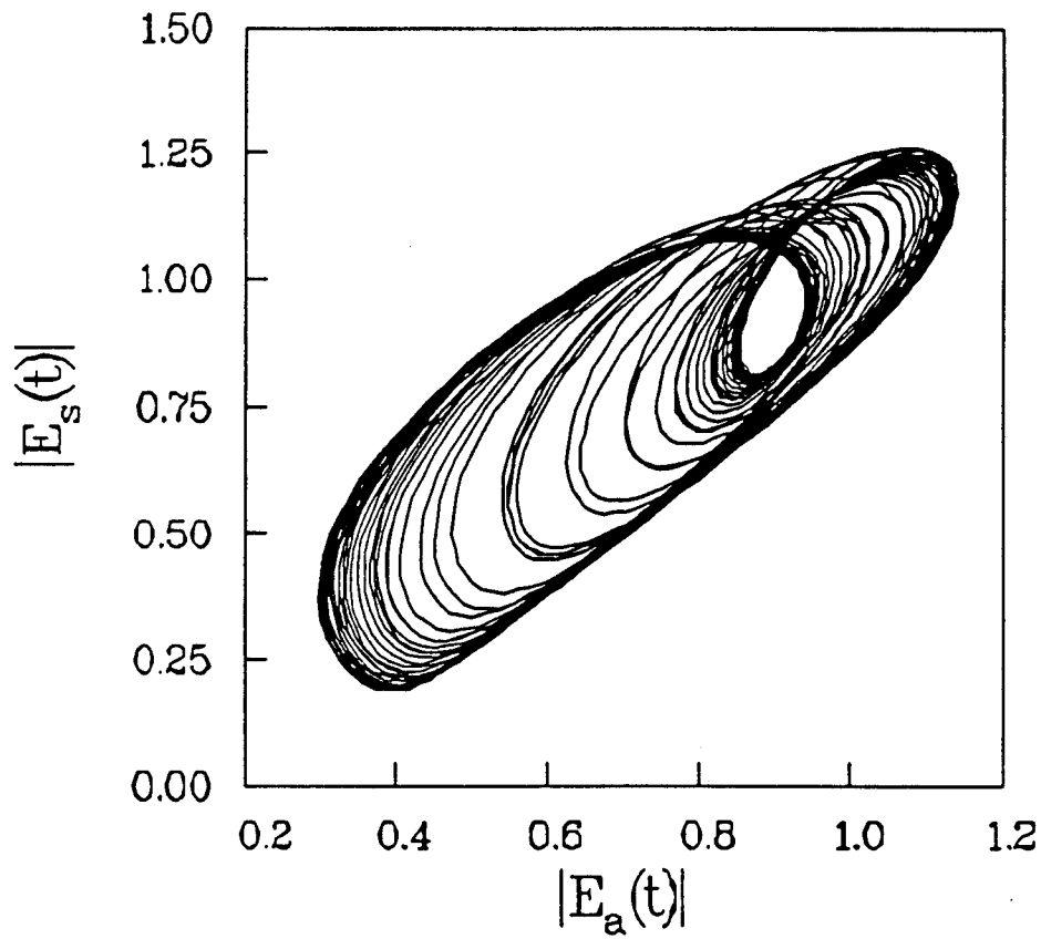
FIG. 7. Quasi-periodic state: Phase portrait at (1.1,1). This state coexists with a periodic state.
