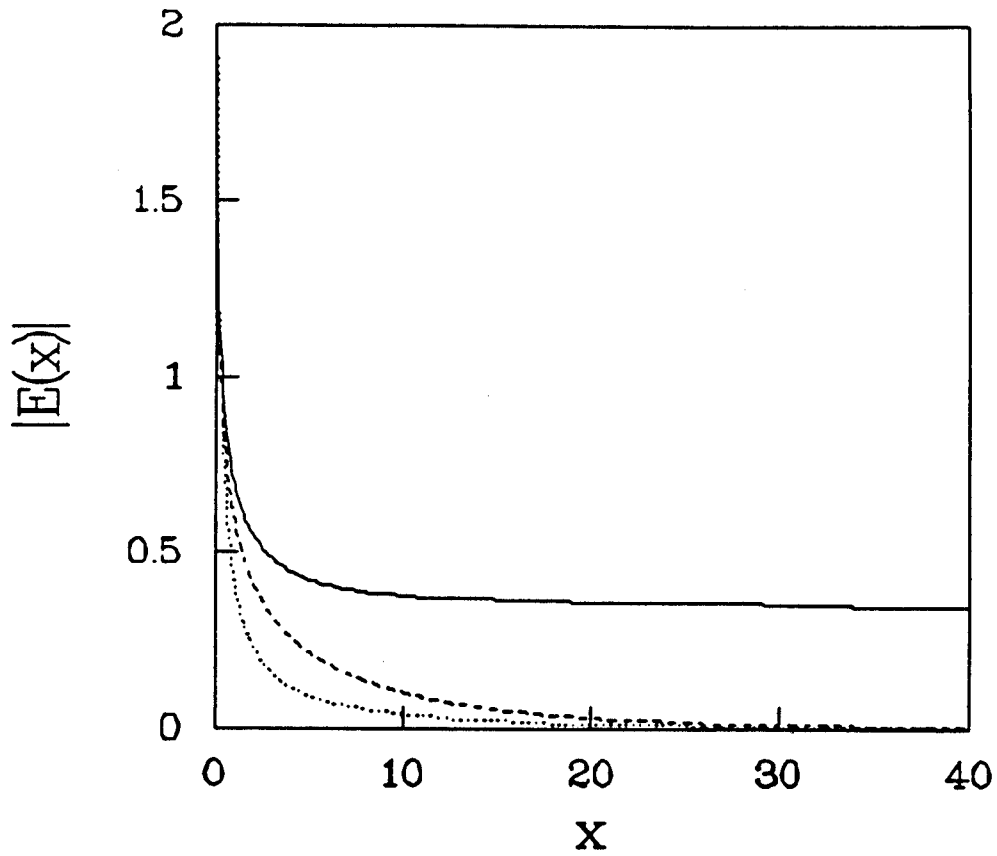
FIG. 2. Fixed state spatial profiles of the pump (solid line), Stokes wave (dashed line) and acoustic wave (dotted line) for the parameters \Delta = 0. , A = 1.6 , L = 20 , \epsilon = 0.0025 .
