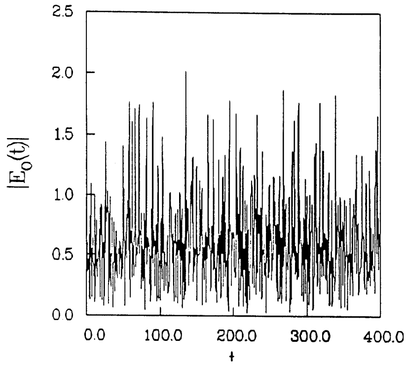
FIG. 9. Chaotic state: Time series of pump at (1,5).
