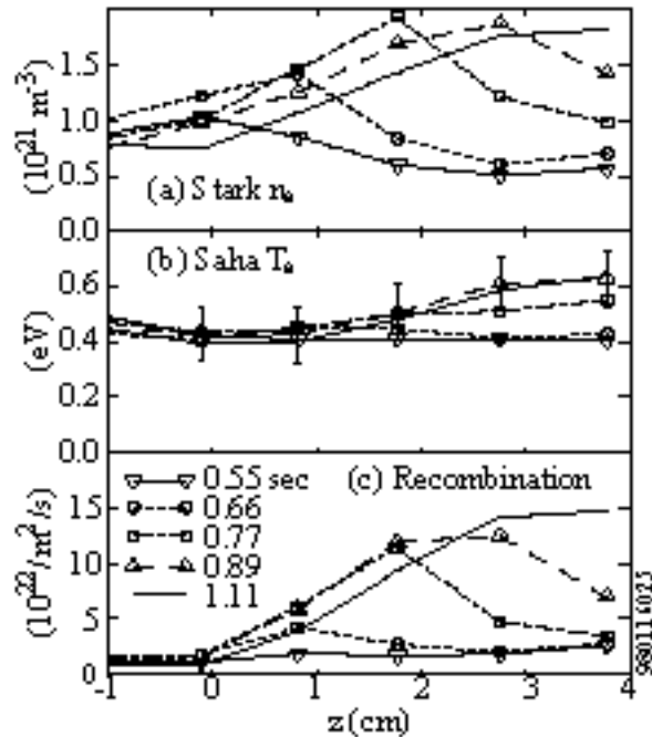
Figure 3: Evolution of the outer divertor characteristics. (a) n_e profiles derived from Stark broadening of Balmer 8 \rightarrow 2 line; (b) T_e derived from fit of Saha distribution to Balmer population densities ( 5 \rightarrow 8 ); (c) Local recombination rate based on n_e , T_e , D_V intensity, assumptions of opacity, and recombinations/photon factor [13].
