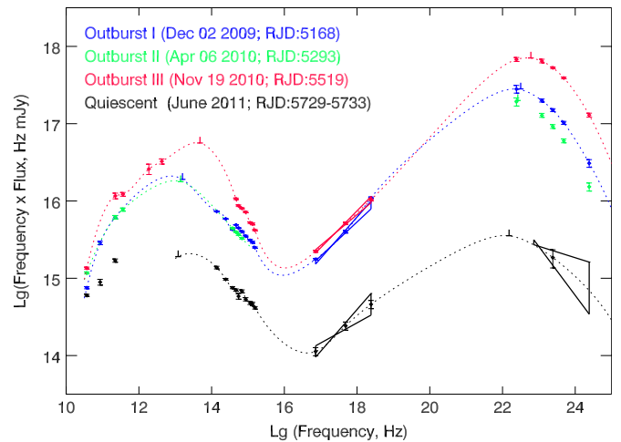
Figure 25. Spectral energy distributions obtained during maxima of outbursts I (blue), II (green), III (red), and at a quiescent state (black); the symbol “┘” denotes low- and high-energy peaks of the SEDs according to modeling (see text Section 5.5), while dotted lines show spline approximations of the data points.
