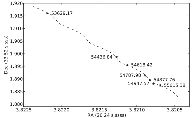
Figure 1. Position of V404 Cyg at each of our seven epochs of observation. Dashed line shows the best-fit proper motion and parallax. Over time, the source moves southwest on the sky (from top left to bottom right of the figure). Each position is labeled with the MJD of the mid-point of the observation.
