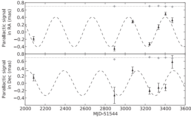
Figure 2. Parallax signature of V404 Cyg in right ascension and declination. The best-fit position and proper motion have been subtracted from the measured astrometric positions. The gray points show the displacement of the check source from its weighted mean position (dotted line), shifted by 0.7 mas for clarity, and scaled by a factor 1/7 to correct for its relative distance from the phase-reference source. This illustrates the scale of the systematic errors.
