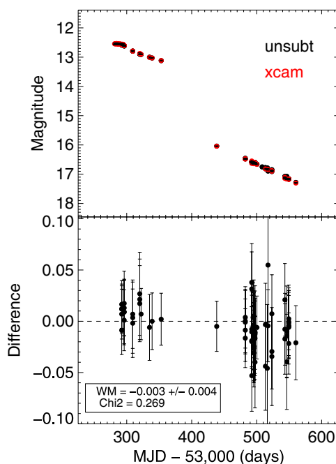
Figure 9. Comparison of the unsubtracted and cross-camera subtracted V-band light curves of SN 2004et.
