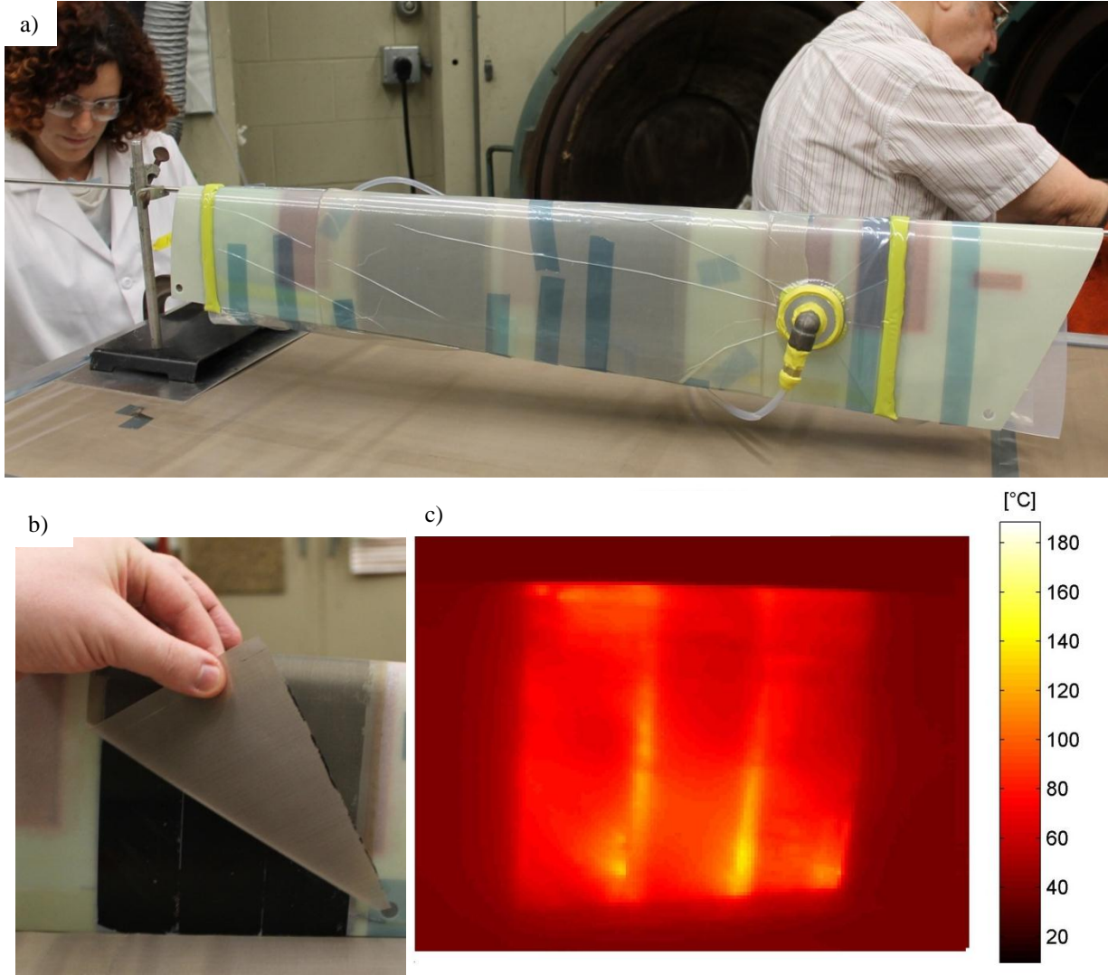
Fig. 5: IPS integration on aerosurface: a) The assembly in a vacuum bag just prior to curing. b) Unpacking the nanostitched IPS after successful cure. c) Thermal image of a preliminary heating experiment.
