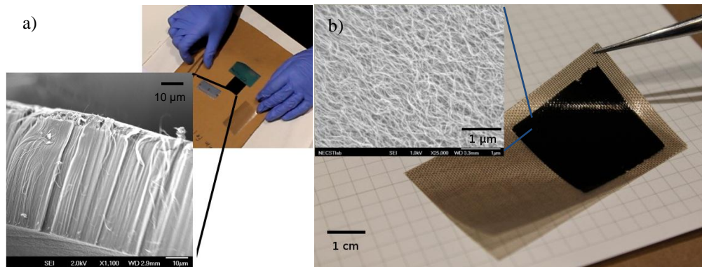
Figure 4: Fabricated knocked-down nanostitch: a) Scanning electron microscopy image illustrating the morphology of a vertically aligned array of CNTs after synthesis and before densification. The height of the shown array is shorter than the material used in the device, which was between 80\ \mu\text{m} and 100\ \mu\text{m} CNT lengths. b) Scanning electron microscopy image showing the morphology of a knocked-down nanostitch layer (inset) and optical image of a small patch on Teflon sheet.
