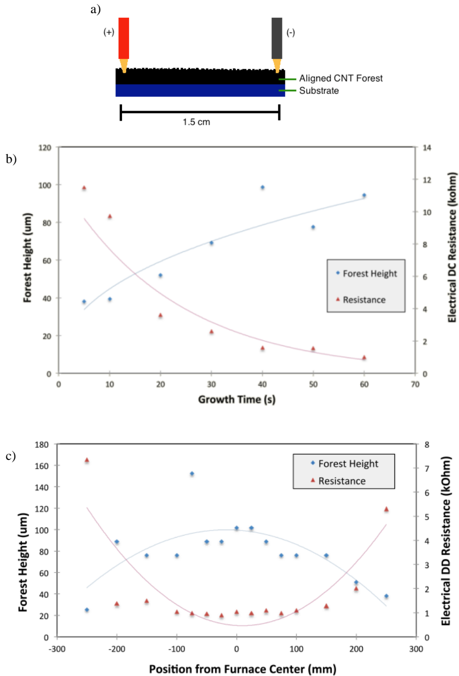
Fig. 1: Aligned-CNT properties used in IPS: a) Schematic of 2-point resistance measurement performed on the CNT forests, using a digital multimeter and spring loaded gold plated contact pins for electrodes, b) CNT forest height at the furnace center for different synthesis times, and the corresponding electrical resistance as measured with a digital multimeter, and c) Different CNT forest growth heights at a range of locations in the furnace for a growth time of 60 s, the growth duration used here for the IPS.
