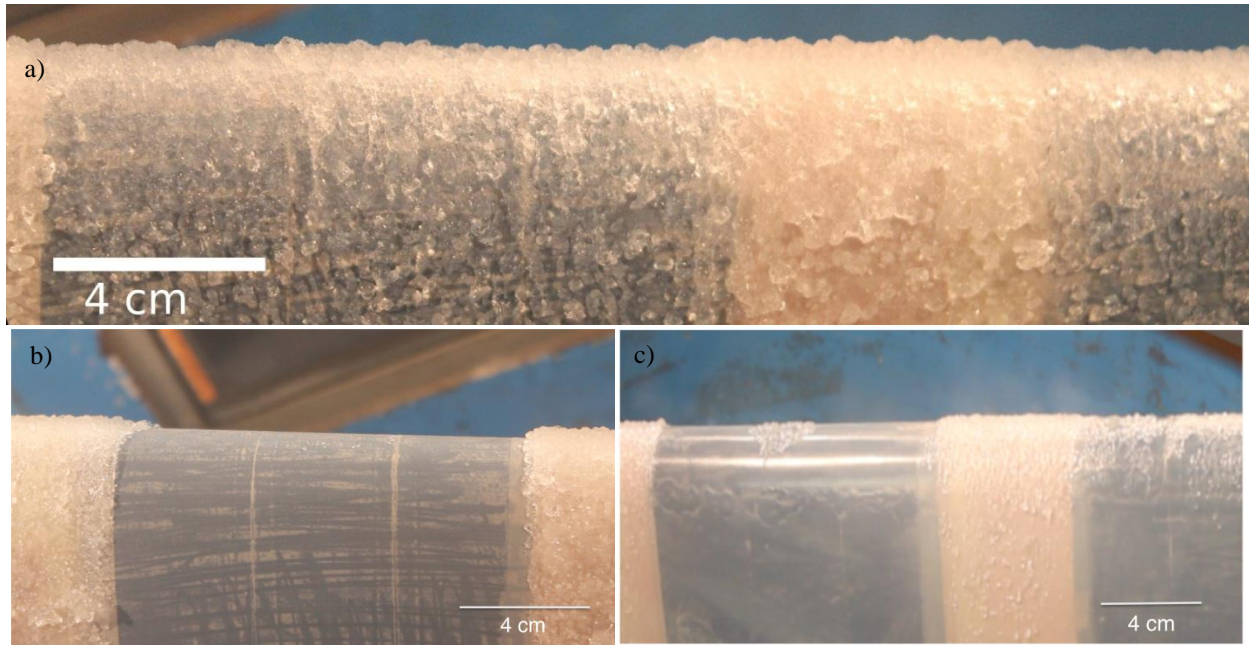
Fig. 6: Optical images from IPS testing in ice tunnel: a) Representative ice accretion after a few minutes of undisturbed exposure with deactivated electrothermal device. b) Aerosurface after successful de-icing. c) Aerosurface during anti-icing.
