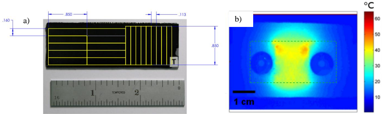
Fig. 2: Polymer nanocomposite IPS preliminary testing: a) knockdown aligned CNT layer cured on an epoxy film adhered to a glass slide. The rectangular delineations indicate individual electrical-resistance test samples. These samples were contacted at the side faces with silver paint and characterized using a digital multi-meter, and b) A low power experiment shows heat distribution across an aligned CNT layer (dashed rectangle) in an epoxy film mounted on a glass fiber reinforced plastic composite sample. The dark round shapes represent rivets, with their centers approx. 30 mm apart, that served as electrical contacts.
