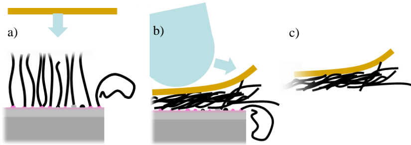
Figure 3: Knocked-down nanostitch fabrication: a-c) Schematic of the knock down procedure consisting of applying the Teflon sheet, compressive shear densification, and lift off of the densified CNT array.
